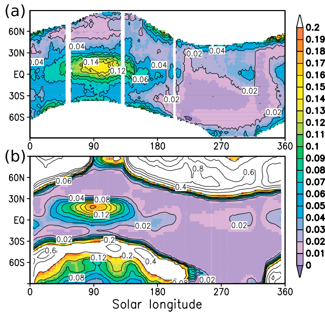
Figure 1. (a) Annual evolution of the zonal mean water ice absorption optical depth at 825\text{ cm}^{-1} ( 12.1\ \mu\text{m} ) as retrieved by TES. (b) Optical depth simulated by the LMD/MGCM. In both cases, year is MY26 and local time is 2 PM. TES cannot retrieve the water ice opacity in the polar regions, where the GCM predicts thick clouds.
