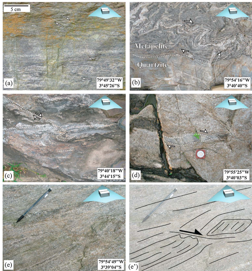
Figure 11. Field-scale photographs of the D_1 deformation-related structures. (a) Photograph of a migmatitic contact at the northern boundary of the Marcabeli granitoid. In the x - z plane, folded leucosome and melanosome and CS structures show a synmetamorphic dextral sense of shear indicating syntectonic dextral emplacement of the Marcabeli granitoid. (b) Photograph of partially molten layers in the upper La Bocana unit in the x - z plane. The photograph shows heterogeneous strain pattern between undeformed quartzitic layers and partially molten metapelite layers with a dextral sense of shear marked by leucosome layers. The white arrow shows the magma pathway direction through the quartzitic layer. (c) Dextral transpressive ductile shear zone at the top of the lower La Bocana unit in the x - z plane. The southern block exhibits centimetric folding compatible with a dextral transpressive sense of shear. (d) Sheared quartzitic xenolith in garnet-bearing mesocrate diatexite of the lower La Bocana unit. Either simple or pure shear can explain the structure depending on the primary orientation of the xenolith with respect to the main stress direction. (e) Magmatic foliation in the Piedras gabbro unit. Melagabbro layer within leucogabbro layers are disrupted and show a dextral sense of shear. Blue arrows: same as in Figure 6.
