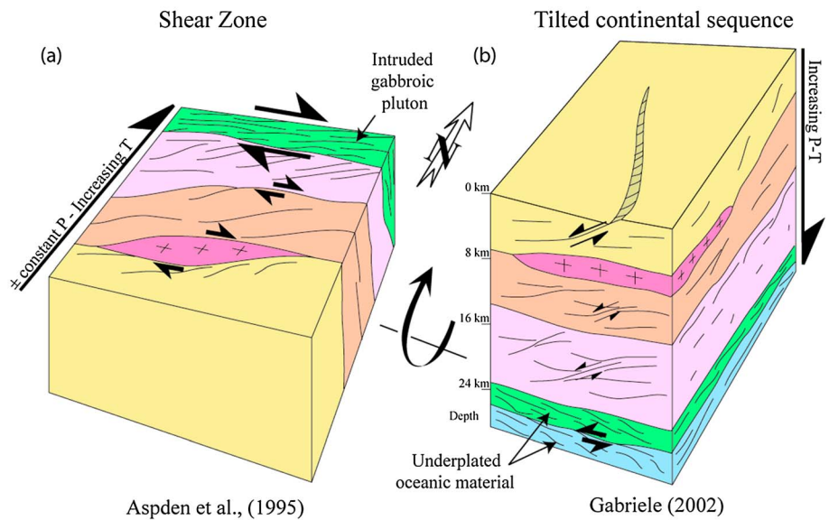
Figure 3. Schematic 3-D diagrams of the El Oro metamorphic province during Late Triassic times. (a) Dextral shear zone model of Aspden et al. [1995]. In this model, emplacement of the gabbroic Piedras unit in a vertical crustal shear zone triggered partial melting and emplacement of the Marcabeli and El Prado granitoid plutons. (b) Model of continental sequence partially molten during Late Triassic times [ Gabriele , 2002]. In this model, the Piedras and the Arenillas-Panupali units represent two distinct episodes of oceanic underplating, and the whole section was tilted during Late Triassic times. Same color chart as for Figure 2.
