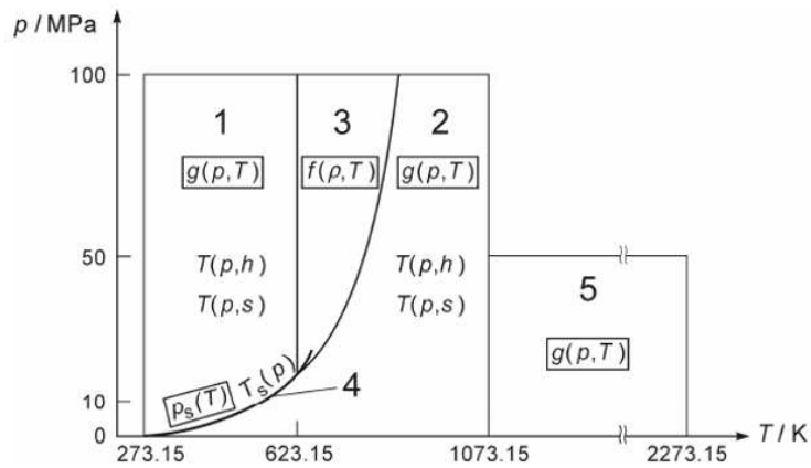
Figure 1: Region of validity for IAPWS-IF97
