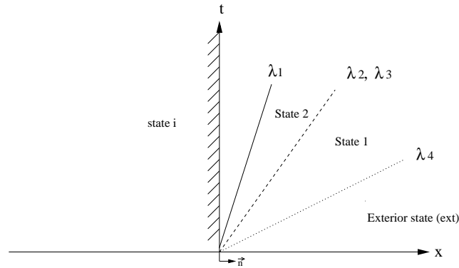
Figure 6: Riemann problem at the outlet, supersonic conditions
