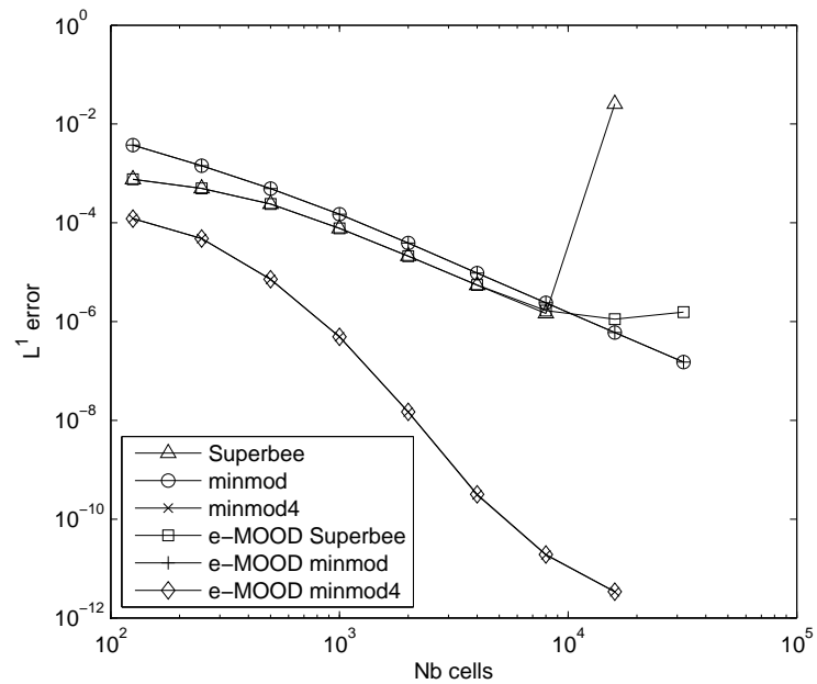
Figure 6: Comparison between MUSCL scheme and e-MOOD scheme – L^1 error for the smooth problem
