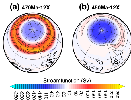
Figure 8. Siberia’s northward drift and the consequences on the longitudinal stream function. Eastward stream is positive (red), westward stream is negative (blue). The stream function is integrated over the whole water column. S: Siberia. Simulations were conducted with the fully coupled version of FOAM. It is noteworthy that the northward drift of Siberia from the Middle to the Late Ordovician is a robust feature of all available Ordovician paleogeographical reconstructions published so far, including the maps from Torsvik and Cocks (Cocks and Torsvik, 2007, Fig. 6a; Torsvik and Cocks, 2013: Fig. 2.12, 2.14 and 2.15), Golonka and Gaweda (2012, Figs. 6 and 7) and Scotese and McKerrrow (1991, Figs. 4 and 5).
