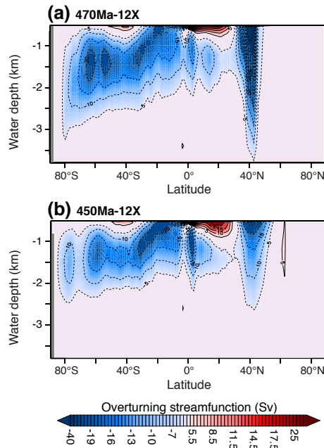
Figure 10. Comparison of the global meridional overturning circulation simulated at 12 PAL with the fully coupled version of FOAM for the two continental configurations used in this study. Red shading and solid contours indicate a clockwise circulation, blue shading and dashed contours indicate a counter-clockwise circulation.
