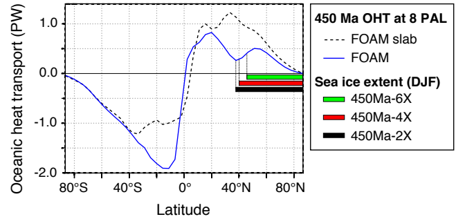
Figure 12. Comparison of the total OHT at 450 Ma and at 8 PAL for the slab version of FOAM and for the fully coupled version of FOAM. The OHT pattern is relatively stable when \text{CO}_2 is varied. Color bars represent the maximum (boreal winter) Northern Hemisphere sea ice extent simulated within the cold climatic mode at 450 Ma with the fully coupled model.
