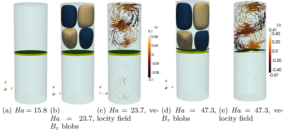
FIGURE 20. Taylor instability in a LMB: (a) Initial condition (b)-(c) t = 4000 and (d)-(e) t = 4050 . B_z contours visualize \pm 10\% of the maximum and minimum value, velocity field plots are colored by U_z . The top and bottom interfaces are visualized by isosurfaces \Phi_1 = 0.5 (yellow or light gray) and \Phi_2 = 0.5 (green or black).
