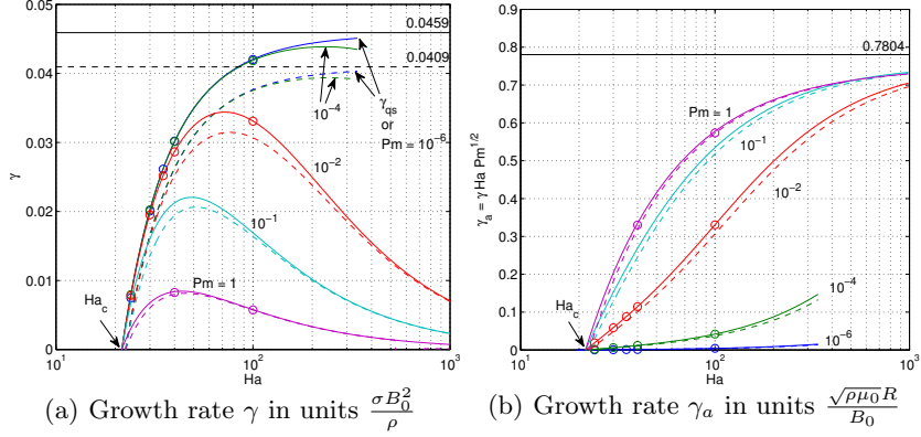
FIGURE 12. Growth rates vs. Ha for various Pm as indicated in the figure using different units. Dashed lines: configuration I. Full lines: configuration II. Markers ( \circ ): growth rates from SFEMaNS. Horizontal lines: non-viscous QS asymptotes in (a), non-viscous non-diffusive asymptote in (b).
