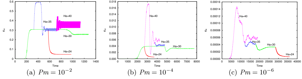
FIGURE 4. Time evolution of the kinetic energy K_\alpha for h = 2 with periodic TB-BC and different Pm as indicated: Ha = 24 (red line), Ha = 30 (green line), Ha = 35 (blue line), Ha = 40 (pink line).
