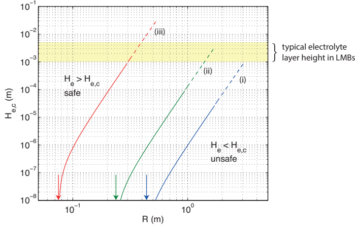
FIGURE 17. Critical height of the electrolyte layer H_{e,c} vs. R for three current density J_0 -scenarios : (i) J_0 = 3 \times 10^3 Am^{-2} , (ii) J_0 = 10^4 Am^{-2} , (iii) J_0 = 10^5 Am^{-2} . Dimensions are in meters. Dashed lines correspond to the high Hartmann number range: Ha \in [300, 1000] (calculated using the asymptotical value of \gamma_{nvqs} ). Arrows indicate critical battery sizes R_c .
