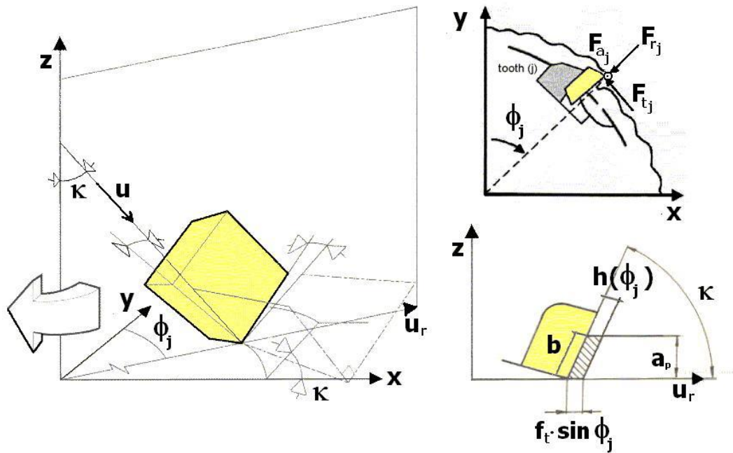
Figure 1. Cutting geometry.
