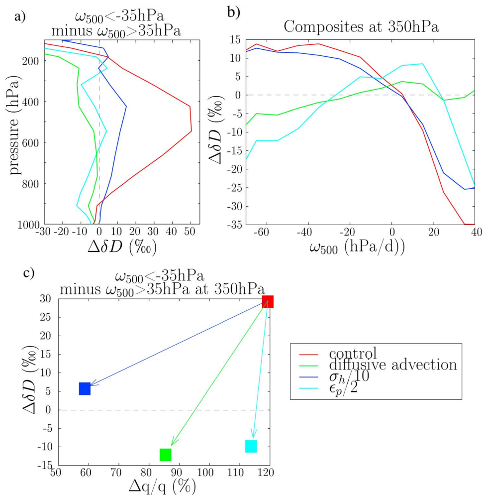
Figure 7. Comparison of water vapor \delta D simulated by the control simulation and the by three moist bias simulations, binned into dynamical regimes. (a) Vertical profiles of the difference between composite of monthly mean \delta D in regions of large-scale ascent (tropical grid cells where \omega_{500} < -35 hPa/d) and composite of monthly mean \delta D in subsidence regions (tropical grid cells where \omega_{500} > 35 hPa/d). The variable \omega_{500} refers to the large-scale vertical velocity at 500 hPa, with negative (positive) values in regions of large-scale ascent (subsidence). (b) Composites of monthly mean \delta D at 350 hPa as a function of \omega_{500} over the tropics. The annual mean, tropical average was subtracted to focus on contrasts between dynamical regimes. (c) Composite of monthly mean \delta D at 350 hPa in convective regions minus that in subsidence regions, as a function of the same difference for q . The difference in q was normalized and expressed in % as follows: (q_{asc} - q_{subs}) / (q_{asc} + q_{subs}) \cdot 200 .
