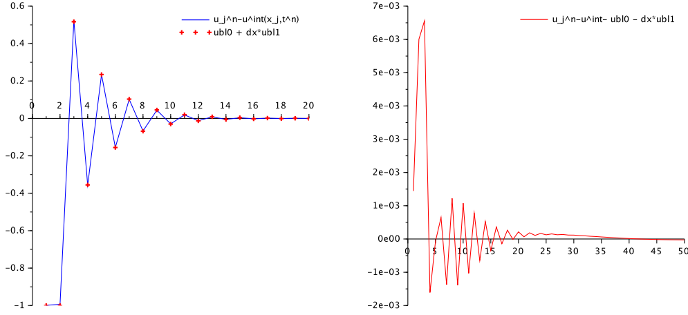
FIGURE 4.3. Boundary layer expansion at time T=0.5 (256 grid points)
