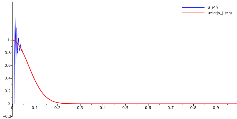
FIGURE 4.2. Numerical solution and exact solution at time T=0.5 (256 grid points).
