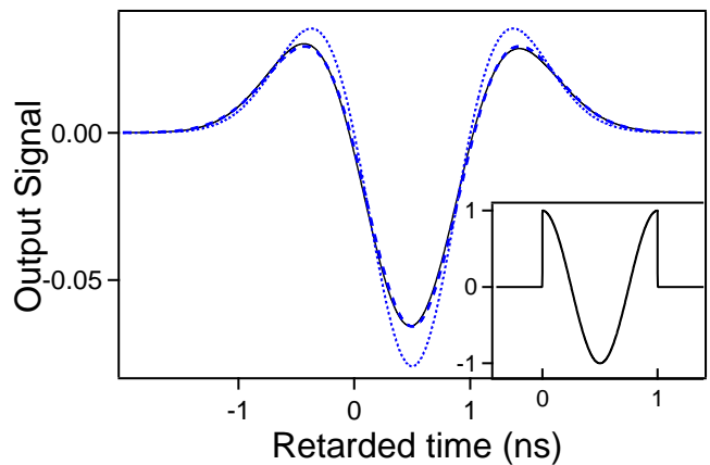
Figure 7: (Color online) Response to the input signal [u_H(t) - u_H(t - T_c)] \cos(\omega_c t) for \alpha_c\ell = 5 . The solid, dashed and dotted lines are the exact FFT solution, the approximate analytical solution given Eq. (29), and the asymptotic solution given Eq. (26), respectively. Inset: input signal.
