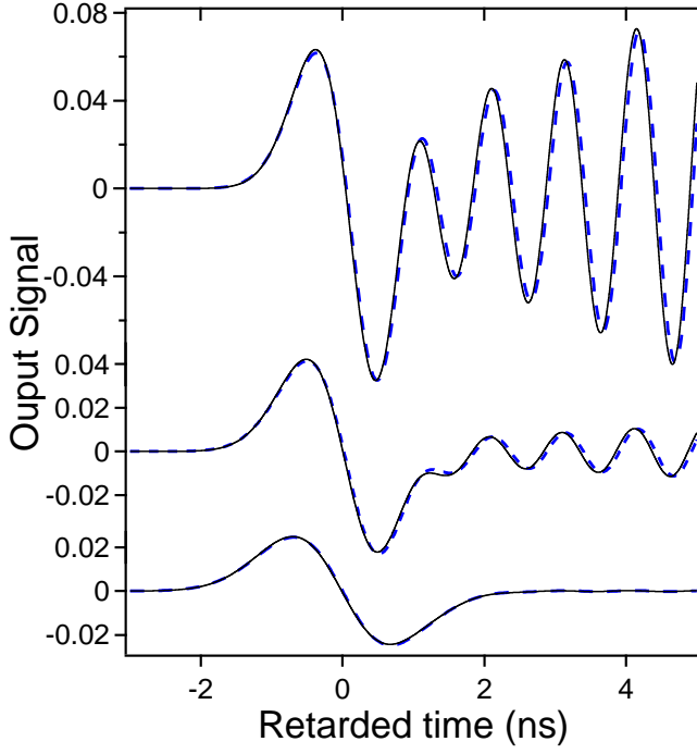
Figure 8: (Color online) Responses to the input signal (t/T_r)u_H(t)\sin(\omega_c t) normalized to 1/(\omega_c T_r) for \alpha_c \ell = 6, 8 , and 12 (from top to bottom). The solid (dashed) line is the FFT exact solution (the approximate analytical solution in terms of error functions).
