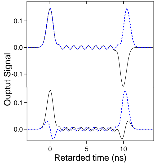
Figure 6: (Color online) Responses to input signals with a long rectangular envelope for \alpha_c \ell = 5 . The upper curves are obtained for v(0, t) \propto \sin(\omega_c t) with T = 10 T_c (solid line) and T = 10.5 T_c (dashed line). The lower curves are obtained for T = 10.25 T_c with v(0, t) \propto \sin(\omega_c t) (solid line) and v(0, t) \propto \cos(\omega_c t) (dotted line). Note that, in the latter case, the postcursor can completely dominate the precursor.
