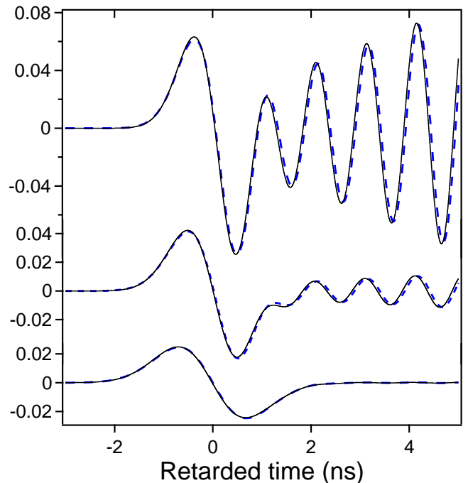
Figure 8: (Color online) Responses to the input signal (t/T_r) u_H(t) \sin(\omega_c t) normalized to 1/(\omega_c T_r) for \alpha_c \ell = 6, 8 and 12 (from top to bottom). The full (dashed) line is the FFT exact solution (the approximate analytical solution in terms of error functions).
