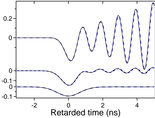
Figure 10: (Color online) Same as Fig.8 with v(0, t) = (t/T_r)u_H(t) \cos(\omega_c t) for \alpha_c \ell = 4.5, 7 and 12 (from top to bottom).
