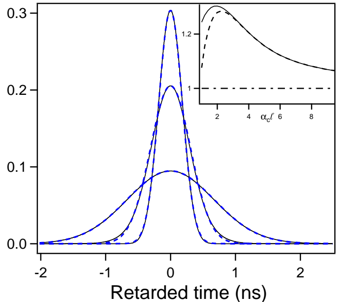
Figure 3: (Color online) Analytical forms of the precursor contribution to the signals of Fig.2 (full lines) and their approximation by the Gaussian given Eq.(15) (dashed lines). Inset : ratios of \beta_p (full line) and A_p (dashed line) over their asymptotic values as a function of the optical thickness.
