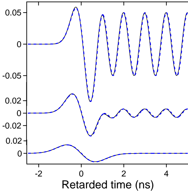
Figure 4: (Color online) Same as Fig.2 when v(0, t) = u_H(t) \cos(\omega_c t) for \alpha_c \ell = 3, 5 and 10 (from top to bottom).
