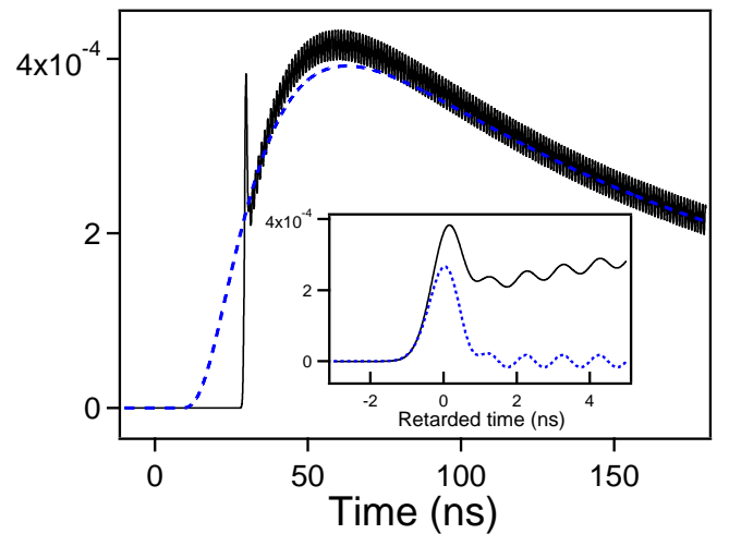
Figure 15: (Color online) Response to the canonical input signal for \sigma \approx 0.3 S/m (other parameters as for the inset of Fig.14). The full (dashed) line is the exact numerical result (the analytical result obtained by considering the sole effects of conductivity). Inset: enlargement of the output signal around t = t_B . Here the dashed line is the analytical result derived from Eq.(48).
