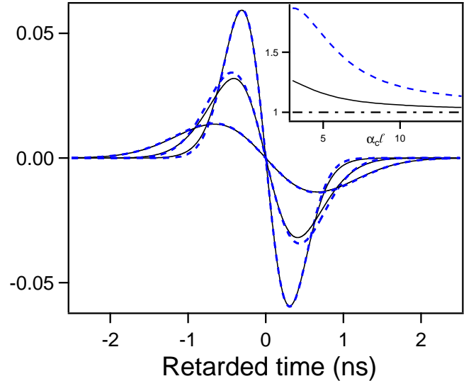
Figure 5: (Color online) Analytical forms of the precursor contribution to the signals of Fig.4 (full lines) and their approximation by the Gaussian derivative given Eq.(19) (dashed lines). Inset as that of Fig.3.
