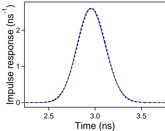
Figure 1: (Color online) Impulse response of deionized water as a function of time for a propagation distance \ell = 10 cm leading to t_B = 2.96 ns and \beta = 4.63 ns ^{-1} . The full [dashed] line is the exact numerical result obtained by FFT [the Gaussian shape given by Eq.(8)].
