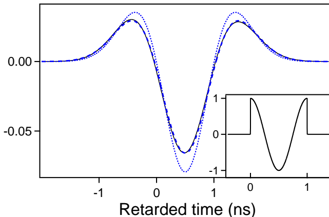
Figure 7: (Color online) Response to the input signal [u_H(t) - u_H(t - T_c)] \cos(\omega_c t) for \alpha_c \ell = 5 . The full, dashed and dotted lines are the exact FFT solution, the approximate analytical solution given Eq.(29) and the asymptotic solution given Eq.(26), respectively. Inset: input signal.
