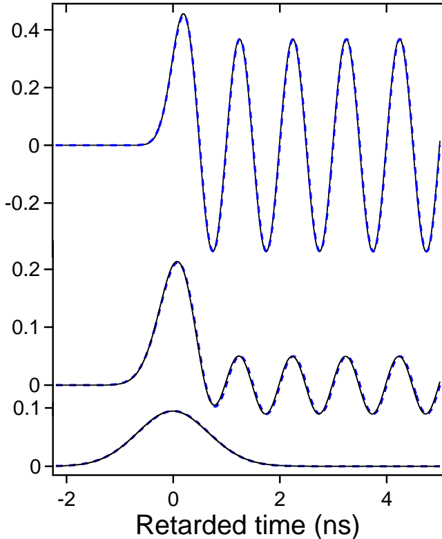
Figure 2: (Color online) Responses to the input signal u_H(t) \sin(\omega_c t) as a function of the time retarded by t_B , for \alpha_c\ell = 1, 3 and 10 (from top to bottom). The full (dashed) lines give the exact numerical solution (our analytical solution in terms of error functions). Note that for the carrier frequency considered ( \omega_c/(2\pi) = 1 \text{ ns}^{-1} ), the optical thickness \alpha_c\ell = 1 is attained for \ell = 21.6 \text{ cm} .
