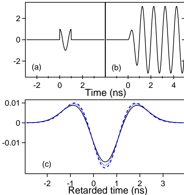
Figure 13: (Color online) Responses to the input signals (a) (full line) and (b) (dashed line) for \alpha_c \ell = 12 . The asymptotic solution of Eq.(44) is given for comparison (dotted line)
