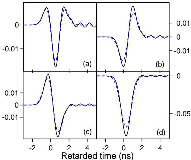
Figure 12: (Color online) Responses (full line) to input signals with trapezoidal envelope of rise times T_r = T_c or T_c/2 for \alpha_c \ell = 7 . (a) T_r = T_c , v(0, t) \propto \sin(\omega_c t) (b) T_r = T_c , v(0, t) \propto \cos(\omega_c t) (c) T_r = T_c/2 , v(0, t) \propto \sin(\omega_c t) and (d) T_r = T_c/2 , v(0, t) \propto \cos(\omega_c t) . The asymptotic solutions (dashed lines) are given for comparison.
