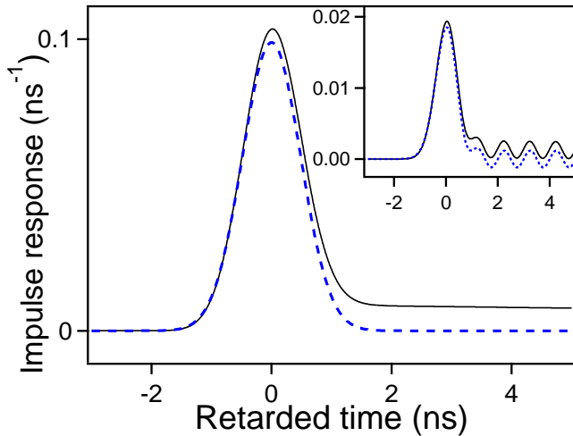
Figure 14: (Color online) Impulse response of water for \ell = 1 m ( t_B \approx 29.6 ns) and \sigma \approx 0.1 S/m. The full (dashed) line is the exact numerical result (our approximate analytical result). Inset: corresponding response to the canonical input signal u_H(t) \sin(\omega_c t) with \omega_c = 2\pi \times 10^9 s ^{-1} .
