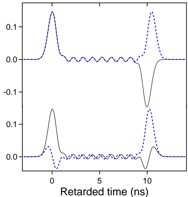
Figure 6: (Color online) Responses to input signals with a long rectangular envelope for \alpha_c \ell = 5 . The upper curves are obtained for v(0, t) \propto \sin(\omega_c t) with T = 10 T_c (full line) and T = 10.5 T_c (dashed line). The lower curves are obtained for T = 10.25 T_c with v(0, t) \propto \sin(\omega_c t) (full line) and v(0, t) \propto \cos(\omega_c t) (dotted line). Note that, in the latter case, the postcursor can completely dominate the precursor.
