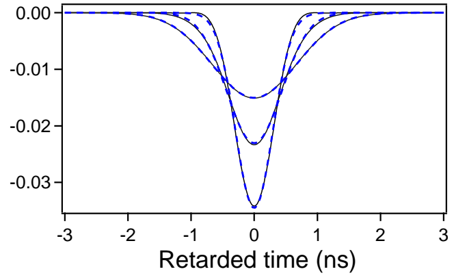
Figure 11: (Color online) Analytical forms of the precursor contribution to the signals of Fig.10 (full lines) and their best fit by Gaussians (dashed lines).
