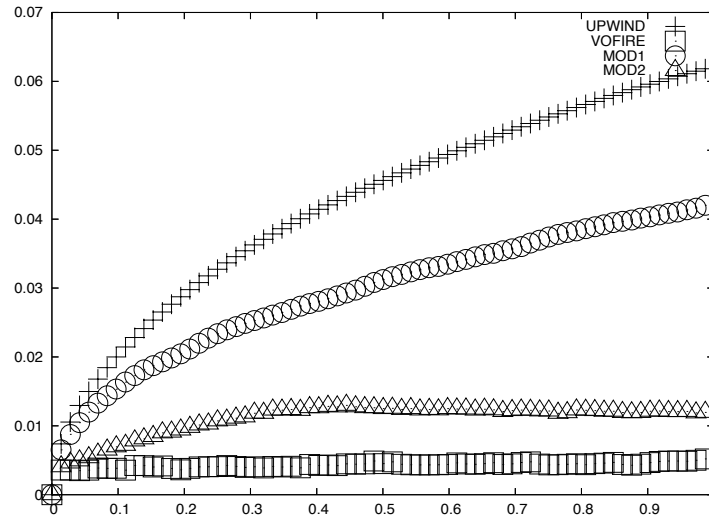
Figure 5: The function t \mapsto F(t) for different schemes. The best curve is the one given by Vofire. Computation done on a triangle unstructured mesh (5996 cells), the Courant number is 0.1. Mod1 (resp. Mod2) corresponds bottom left (resp. bottom right) of figure 4.
