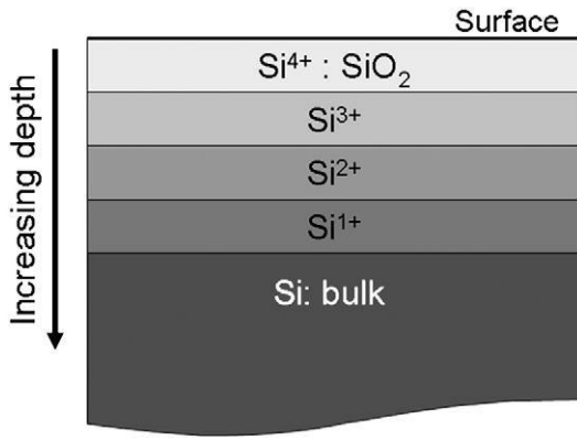
Fig. 10. Schematic of the five-layer model: each layer corresponds to a different chemical state of silicon, going from the substrate (bulk silicon, Si 0 ), through the sub-oxides (Si 1+ , Si 2+ , and Si 3+ ) to the surface (silica, Si 4+ ).
