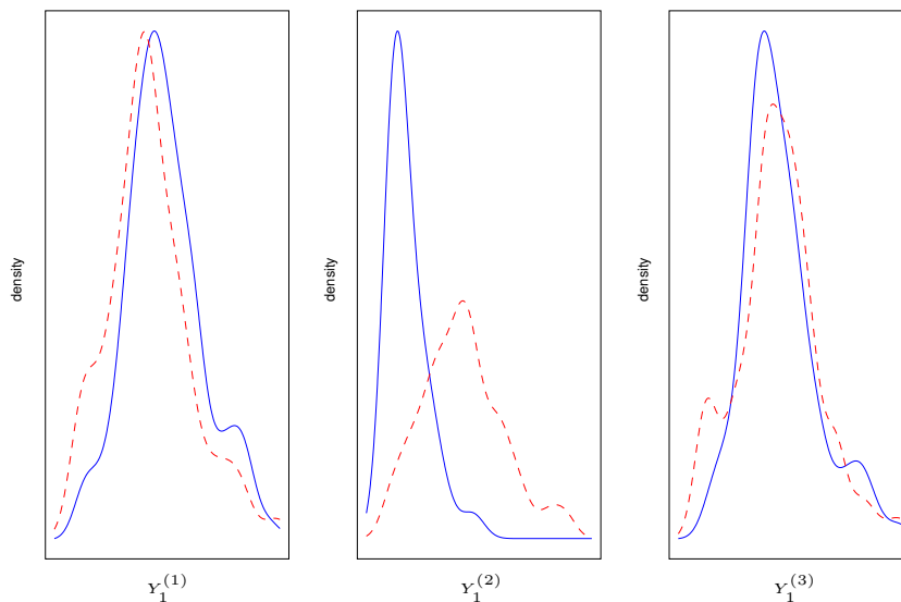
Figure 10: Kernel estimates \hat{f}_1^{(j)} (solid lines) and \hat{f}_2^{(j)} (dashed lines) for j = 1 (left), 2 (center) and 3 (right).
