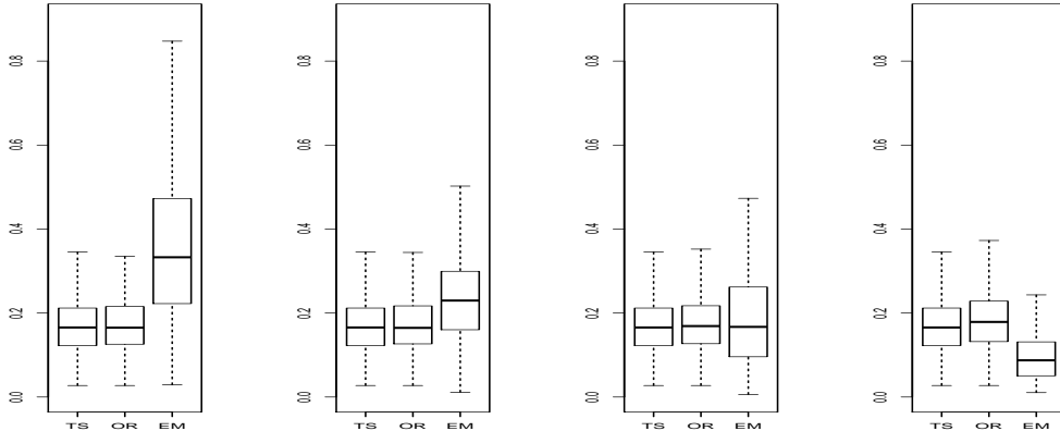
Figure 4: Boxplot of the L_1 -error for the estimate f_1^{em} (EM), the oracle estimate \bar{f}_1 (OR) and the two-step estimate \hat{f}_1 (TS) for the Laplace example. The separation distance \Delta between f_1 and f_2 vary from 0.1 (left) to 2 (right) and \ell_n = 5.5 .
