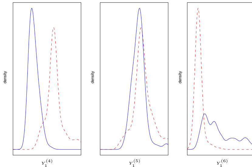
Figure 11: Kernel estimates \hat{f}_1^{(j)} (solid lines) and \hat{f}_2^{(j)} (dashed lines) for j = 4 (left), 5 (center) and 6 (right).
