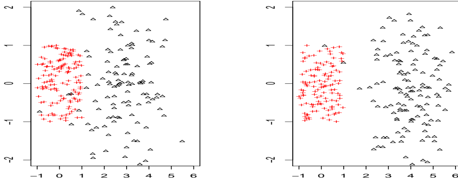
Figure 6: A sample of n = 250 observations for the “Circle-Square” model with a = 3 (left) and a = 4 (right).
