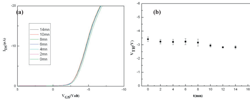
Fig. 5. Stability (a) shift of the transfer characteristic with time; (b) Voltage shift versus time.
