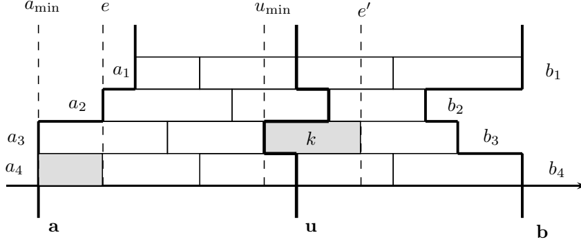
Figure 2: Illustration of Proposition 2
