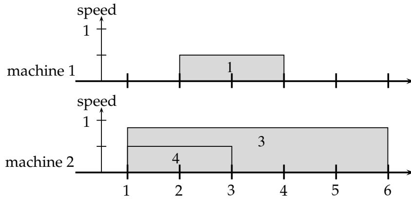
Figure 8: Speed profile v_i(t) at the end of Step 3
