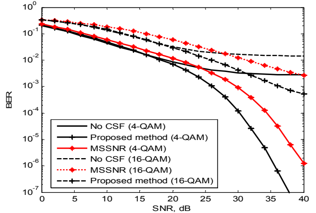
Fig. 9. BER performance versus SNR for C2
