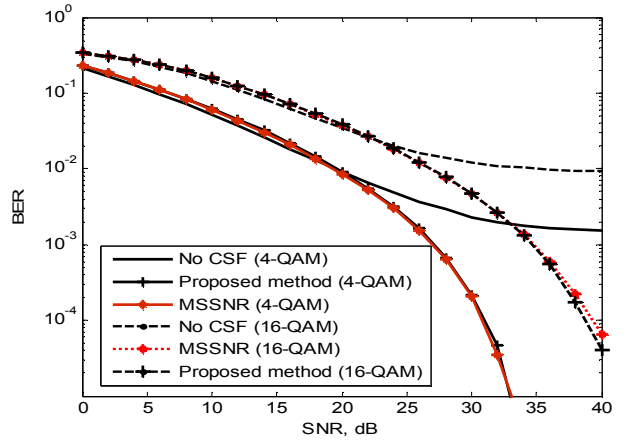
Fig. 6. BER performance versus SNR for C1
