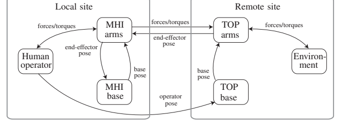
Fig. 3. Coordination scheme considering coupling of bodies and end-effectors
