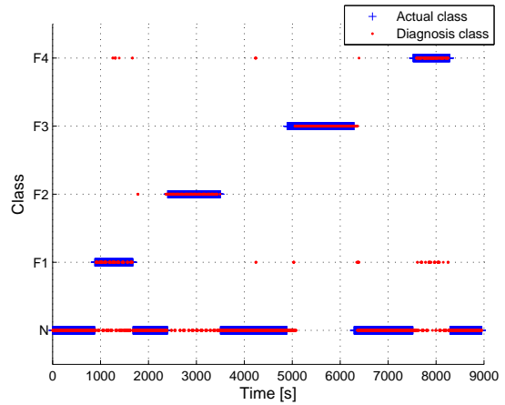
(b) Diagnosis results: training data
