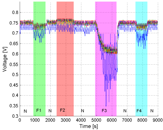
(a) Evolutions of cell voltages: training data
