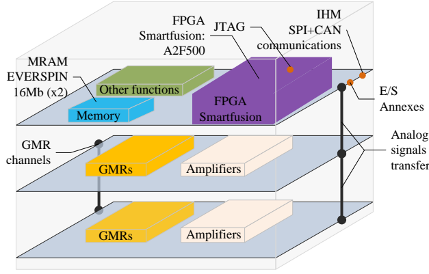
Figure 3: Embedded system designed for PEMFC system diagnosis [8]
