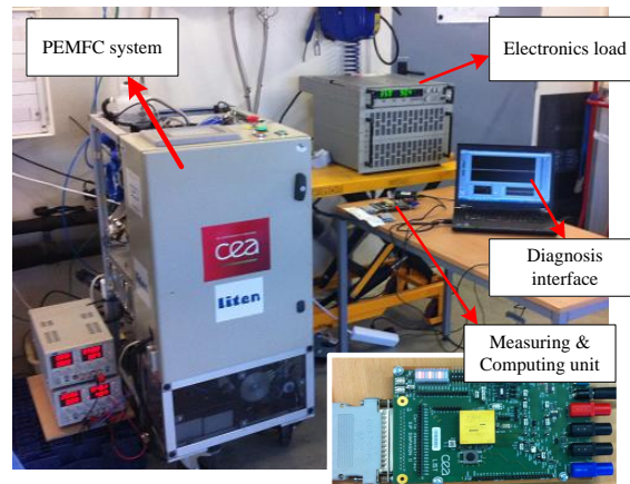
Figure 2: Overview of the developing platform
