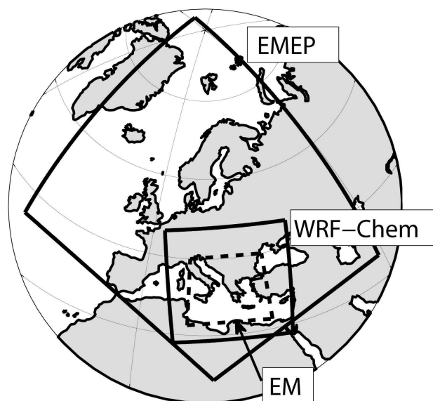
Fig. 1. Locations of the domains used in the EMEP MSC-W and WRF-Chem simulations, and of the study region ( 11\text{--}30^\circ \text{ E} , 32\text{--}45^\circ \text{ N} ) covering most of the Eastern Mediterranean (EM). Coordinates of the four corners of the two model domains are ( 35.8^\circ \text{ W} , 40.5^\circ \text{ N} ), ( 16.7^\circ \text{ E} , 20.3^\circ \text{ N} ), ( 58.6^\circ \text{ E} , 34.8^\circ \text{ N} ) and ( 131.8^\circ \text{ W} , 86.5^\circ \text{ N} ) for EMEP MSC-W, and ( 8.1^\circ \text{ E} , 28.2^\circ \text{ N} ), ( 33.9^\circ \text{ E} , 28.2^\circ \text{ N} ), ( 38.8^\circ \text{ E} , 49.8^\circ \text{ N} ) and ( 3.2^\circ \text{ E} , 49.8^\circ \text{ N} ) for WRF-Chem.
