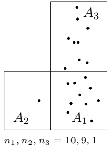
Figure 3: Sample of n = 20 points in a 2-d space, partitioned into three rectangles. As \alpha increases, the minimum volume sets \hat{\Gamma}_\alpha are successively equal to A_1, A_1 \cup A_2, A_1 \cup A_3 , and A_1 \cup A_3 \cup A_2 , whereas, in the EM -approach, as t decreases, the \hat{\Omega}_t 's are successively equal to A_1, A_1 \cup A_3 , and A_1 \cup A_3 \cup A_2 .
