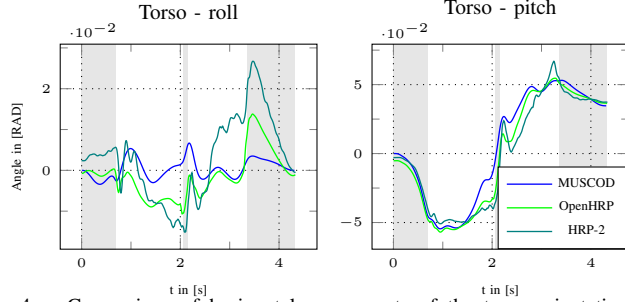
Fig. 4. Comparison of horizontal components of the torso orientation that are computed during optimization (MUSCOD), and estimated in the simulation of the virtual robot (OpenHRP), as well as during the experiment on HRP-2. Whilst the roll angle shows higher deviations the pitch orientation follows nicely the optimization results.
