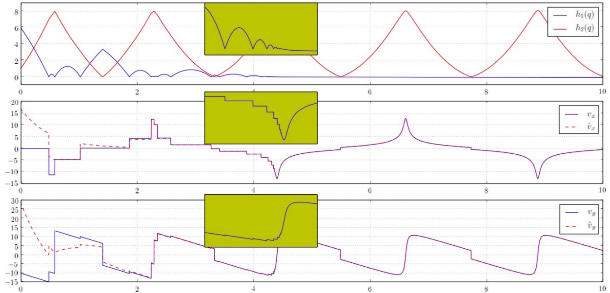
Fig. 5: Velocity estimation for a 2-degree of freedom mechanical system: A ball bouncing inside a parabola with ceiling. The top plot shows the evolution of two gap functions h_1(q) and h_2(q) with time. The middle and bottom plot show the velocity components v_x and v_y , along with their estimates, respectively. The boxes in the center of these plots provides a magnified image of the quantity of interest around the accumulation point t = 4.5s .
