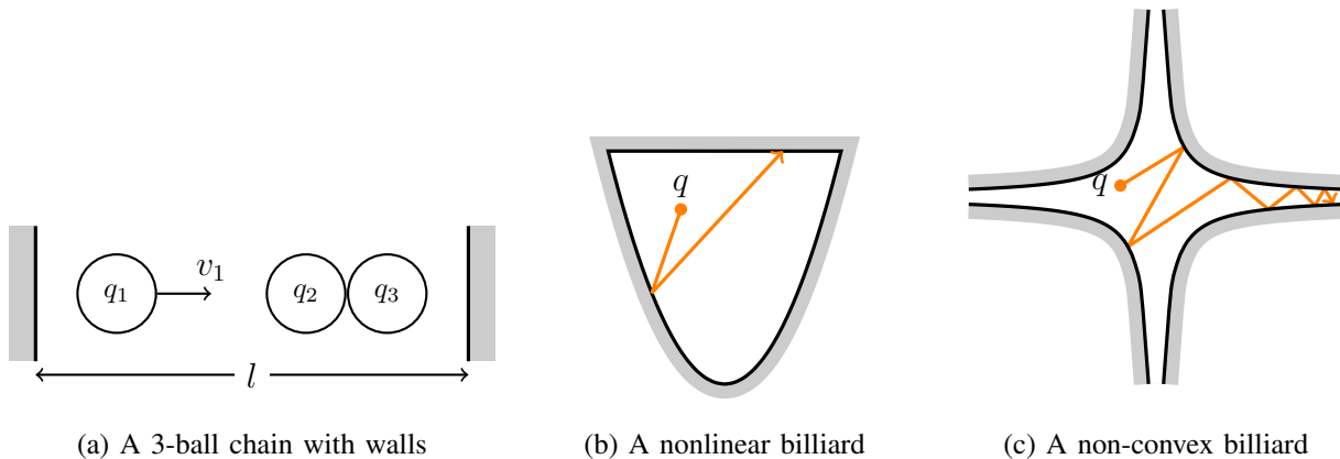
Fig. 1: Examples of systems with unilateral constraints.
