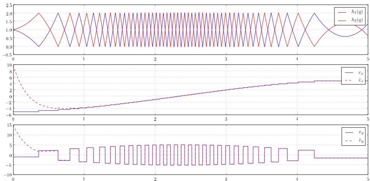
Fig. 7: Simulation of velocity estimator for a particle moving in a nonconvex hyperbolic billiard.
