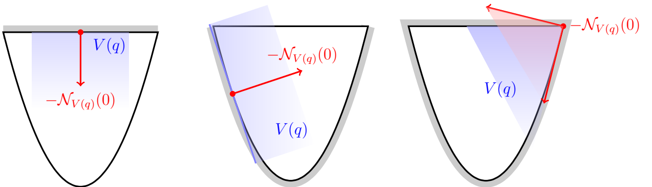
(a) Cones for the case h_1(q) \leq 0 . (b) Cones for the case h_2(q) \leq 0 . (c) Corner case: h_1(q) \leq 0 \wedge h_2(q) \leq 0 .
