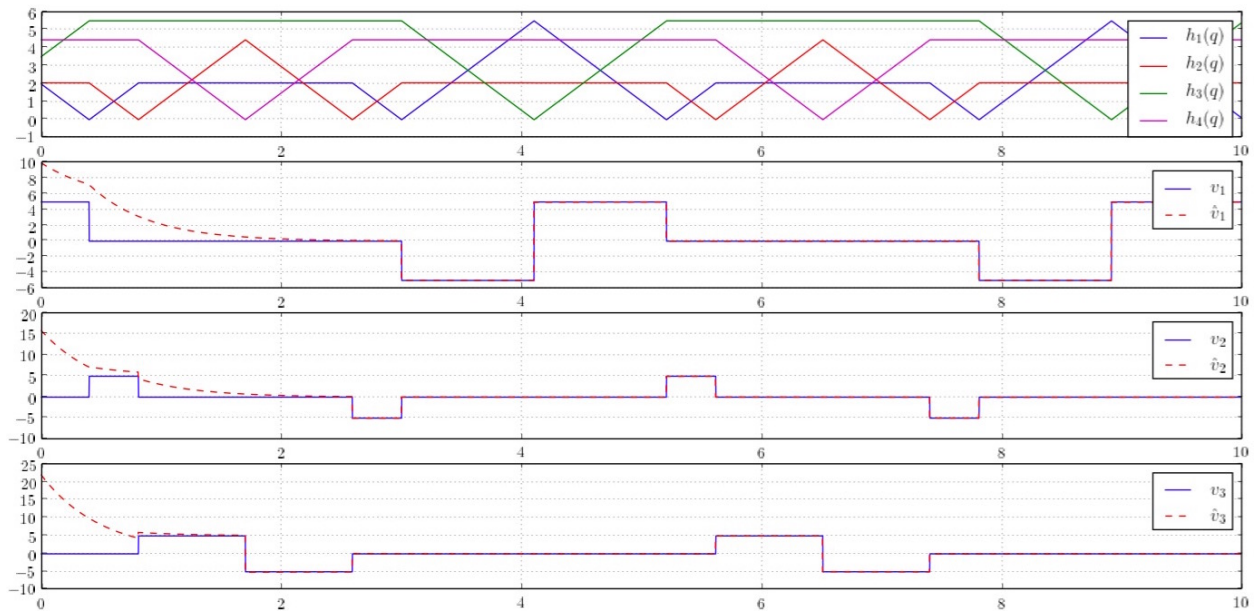
Fig. 4: Simulation of velocity estimator for 3-ball chain with e = 1 , and no external forces.
