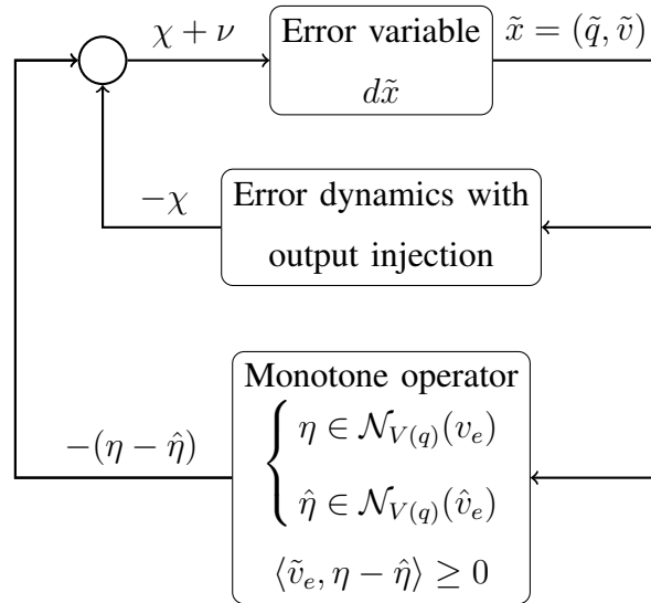
Fig. 3: Interpretation of error dynamics (27) in terms of passivity.
