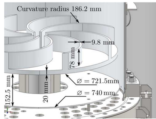
FIG. 2. Geometry of the (lower) impeller and additional aluminium disk below.
