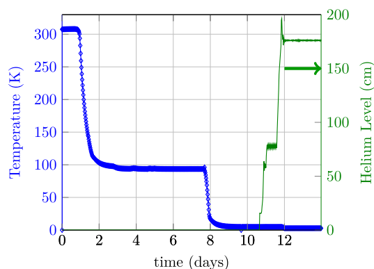
FIG. 9. Cool down. The helium level is measured inside the saturated bath.
