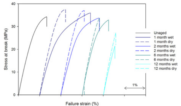
Fig. 4. Evolution of tensile behaviour of PHBV specimens aged at 40°C for different periods, before and after drying.
