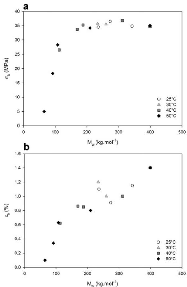
Fig. 9. Evolution of the stress at break (a) and strain at break (b) as a function of molecular weight.
