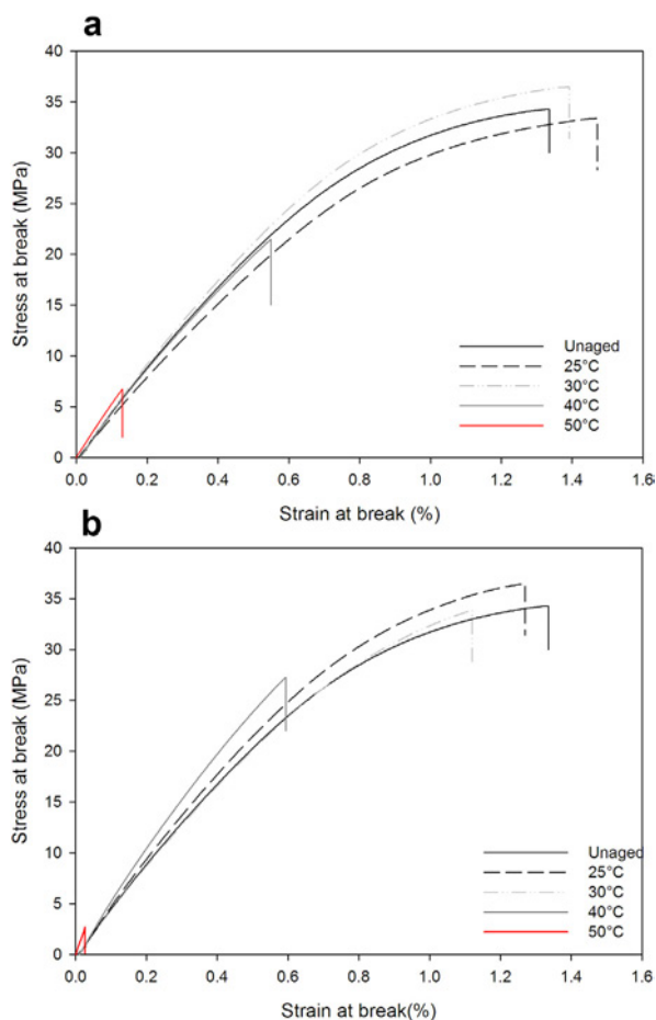
Fig. 5. Evolution of the tensile behaviour of PHBV specimens aged in distilled water at 25, 30, 40 and 50°C after 360 days: before (a) and after drying (b).
