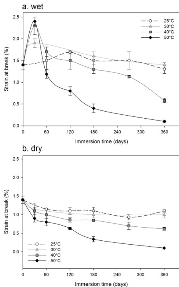
Fig. 7. Evolution of the strain at break of PHBV specimens aged in distilled water at 25, 30, 40 and 50°C after 360 days: before (a) and after drying (b).
