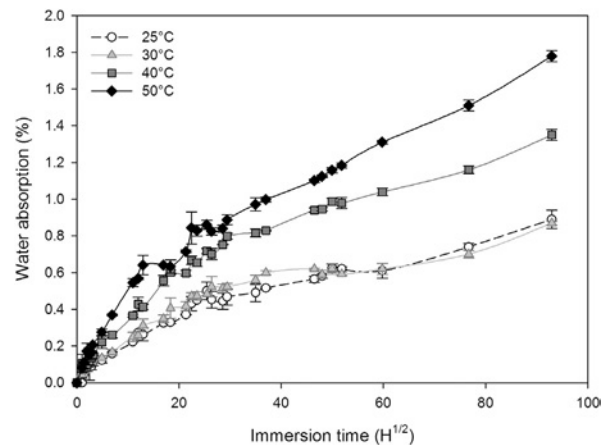
Fig. 1. Evolution of water uptake as a function of the square of root of immersion at different temperatures in distilled water.
