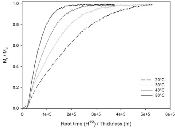
Fig. 2. Plots of M_t/M_\infty against t^{1/2}/\text{thickness} for PHBV at different temperatures obtained by DVS and corresponding at 50% RH.
