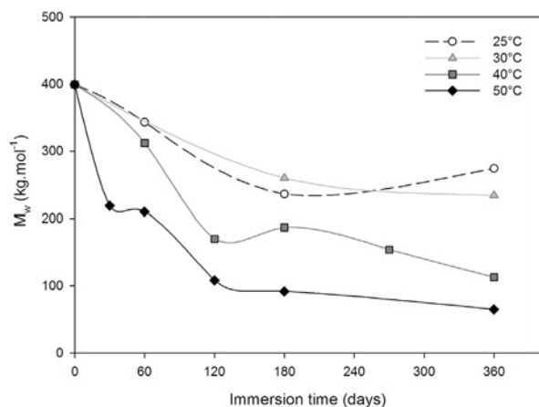
Fig. 8. Evolution of the molecular weight, \bar{M}_w , of PHBV specimens aged in distilled water at 25, 30, 40 and 50°C after 360 days.
