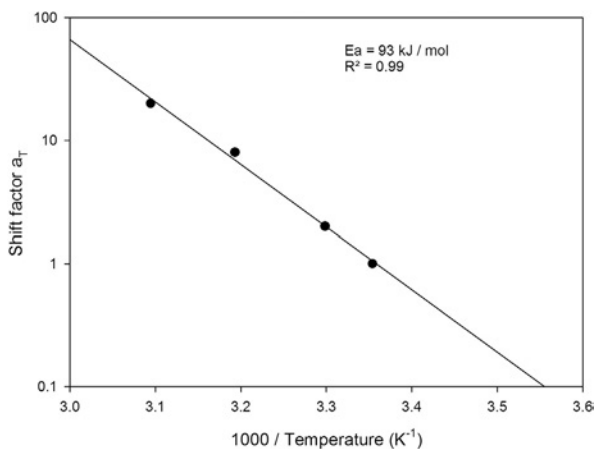
Fig. 11. Identification of the activation energy for the strain at break indicator.
