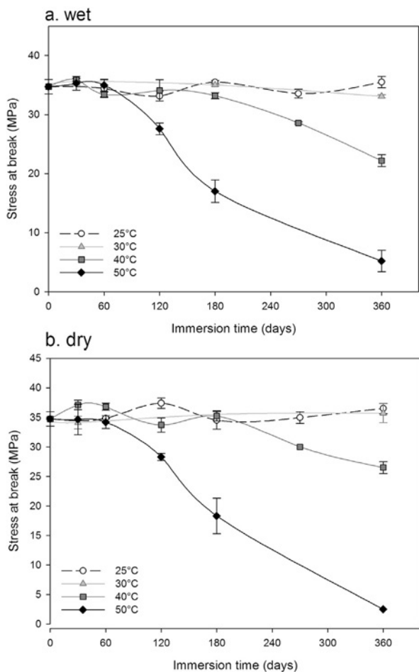
Fig. 6. Evolution of the stress at break of PHBV specimens aged in distilled water at 25, 30, 40 and 50°C after 360 days: before (a) and after drying (b).
