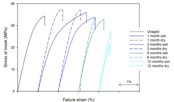
Fig. 4. Evolution of tensile behaviour of PHBV specimens aged at 40^\circ\text{C} for different periods, before and after drying.
