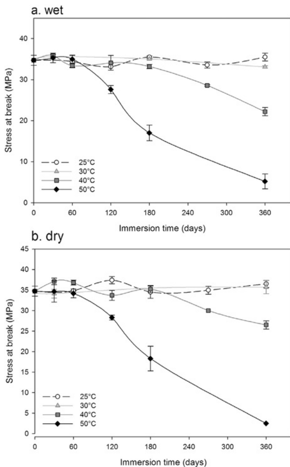
Fig. 6. Evolution of the stress at break of PHBV specimens aged in distilled water at 25, 30, 40 and 50°C after 360 days: before (a) and after drying (b).
