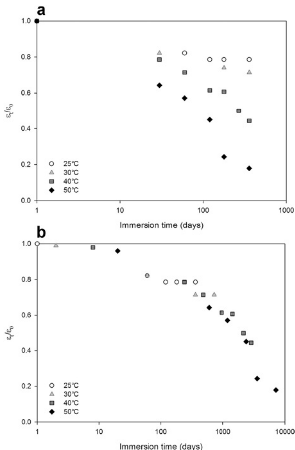
Fig. 10. Evolution of the normalized strain at break as a function of ageing time for all the temperatures (a) and master curve (b).
