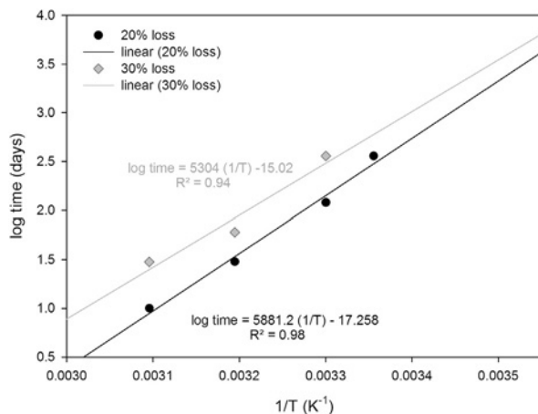
Fig. 12. Evolution of different percentage of loss properties and extrapolation to 13°C in order to predict lifetime.
