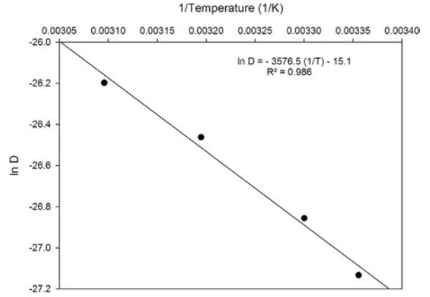
Fig. 3. Identification of the diffusion coefficient of distilled water in the PHBV for different temperatures by DVS.
