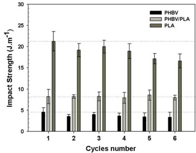
Fig. 8 Impact strength as a function of number of reprocessing cycles for PHBV, PLA and PHBV/PLA blend
