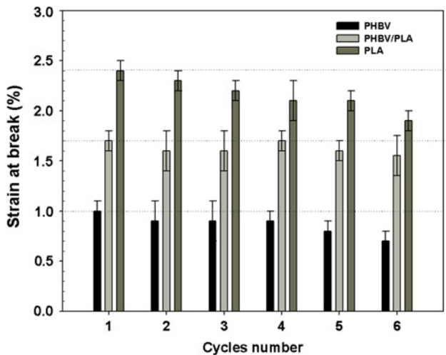
Fig. 7 Strain at break as a function of number of reprocessing cycles for PHBV, PLA and PHBV/PLA blend
