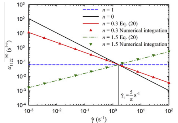
Fig. 3. Variations of the a_{1122}^{(n=1)} and a_{1122}^{(n=0)} components as a functions of shear rate in for simple shear flow. Also shown are the results obtained with Eq. (20) and numerical integration for the case of n = 0.3 and n = 1.5 .
