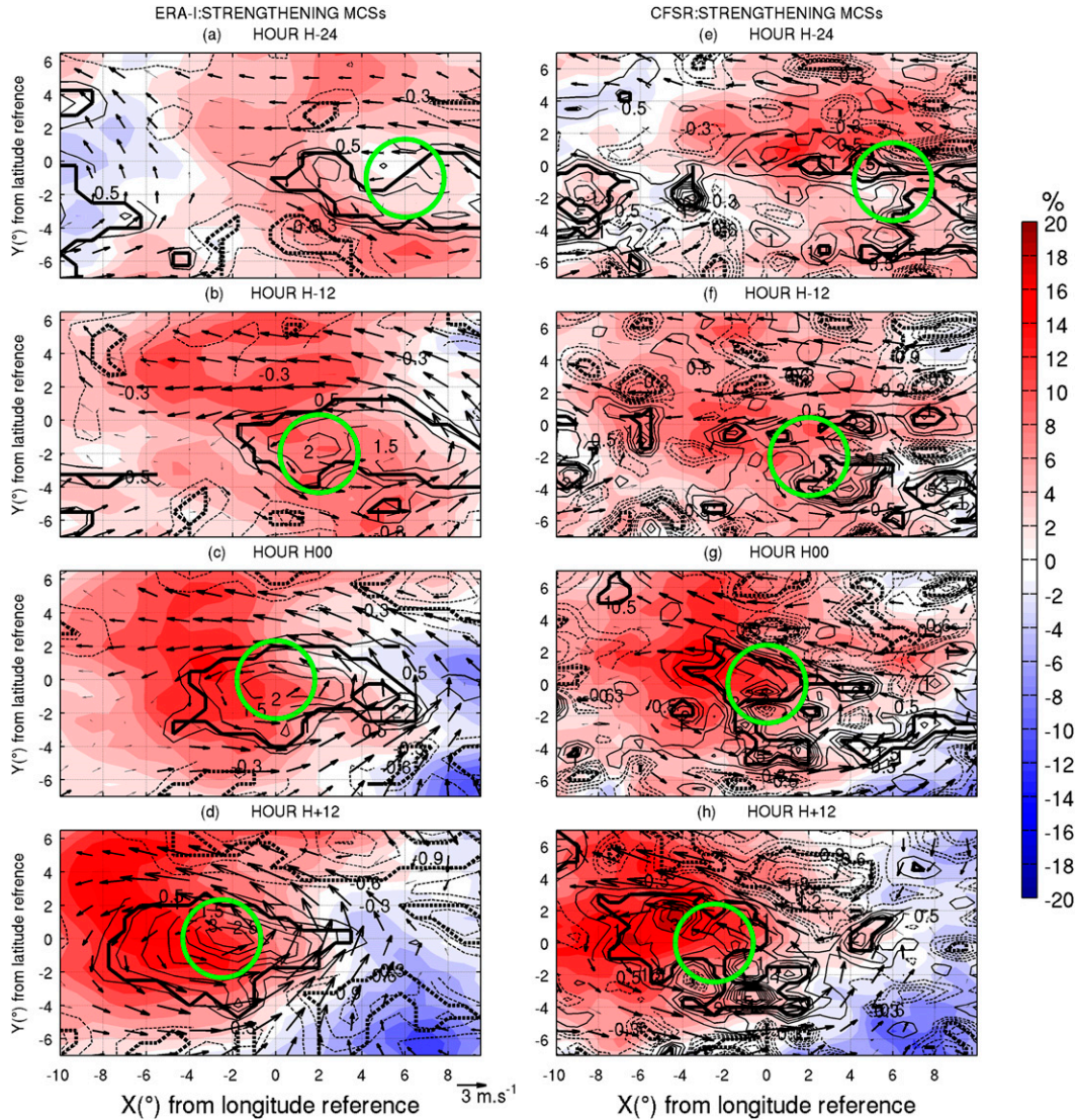
FIG. 6. Composites at 700 hPa of relative humidity anomaly (colors, %), wind anomaly (arrows, \text{m s}^{-1} ), and relative vertical vorticity anomaly (contours, \times 10^{-5} \text{ s}^{-1} ) at (a),(e) H - 24 h, (b),(f) H - 12 h, (c),(g) H00, and (d),(h) H + 12 h with (left) ERA-Interim and (right) CFSR for strengthening MCSs. Significant values are in bold contours for relative vertical vorticity anomaly and in bold arrows for wind anomaly. The horizontal (vertical) axis (in degrees) is the distance from the reference longitude (latitude). The mean position of the MCS vortex center is indicated by the green circle.
