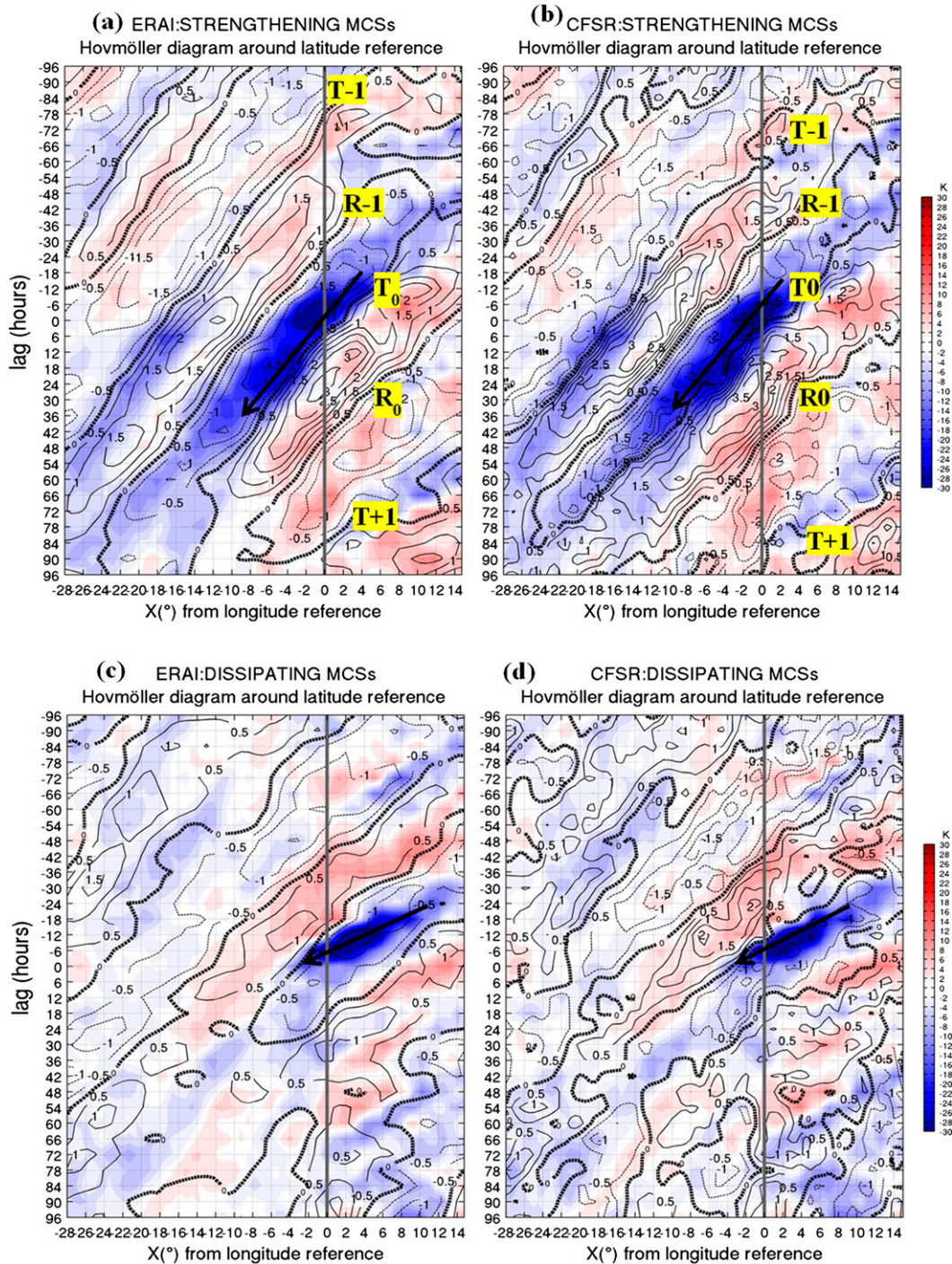
FIG. 11. Hovmöller diagram of brightness temperature anomaly (colors, K) and 850-hPa meridional wind anomaly (contours, \text{m s}^{-1} ) with (left) ERA-Interim and (right) CFSR for the (a),(b) strengthening and (c),(d) dissipating MCS composite. The vertical gray line is the reference longitude, and T (R) shows the trough (ridge) wave position. The bold black arrow shows the approximate propagation direction of the MCS composite.
