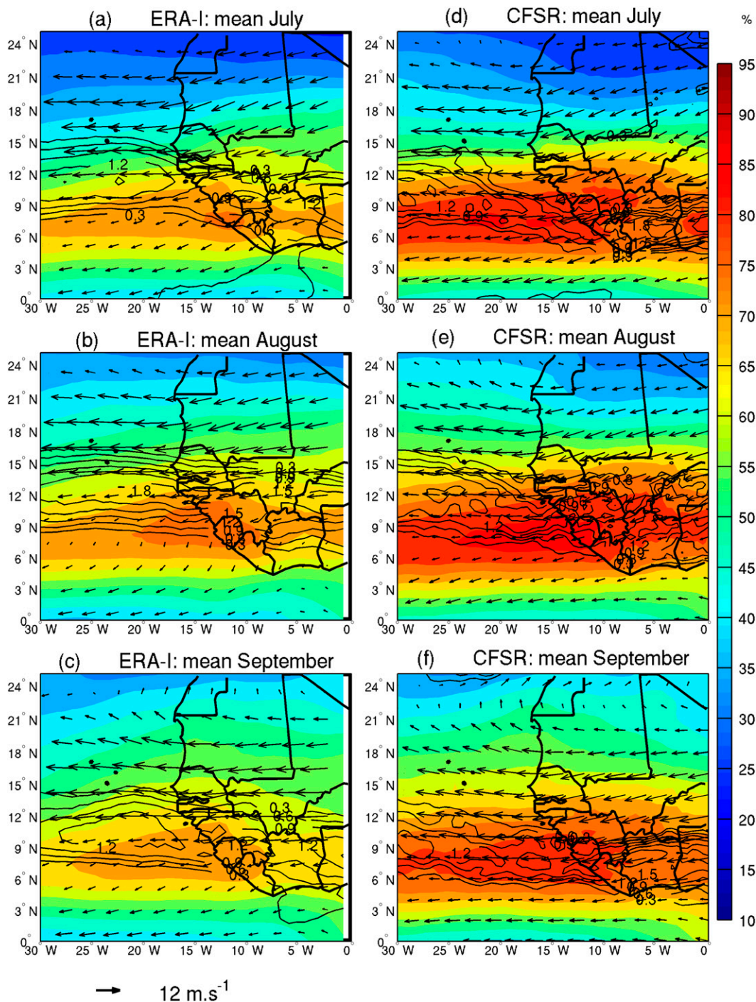
FIG. 3. Mean fields at 700 hPa of relative humidity (colors, %), wind (arrows, \text{m s}^{-1} ), and positive relative vertical vorticity (contours, \times 10^{-5} \text{ s}^{-1} ) of (a),(d) July, (b),(e) August, and (c),(f) September with (left) ERA-Interim and (right) CFSR. The fields were only averaged over the years including the dates of selected MCSs.
