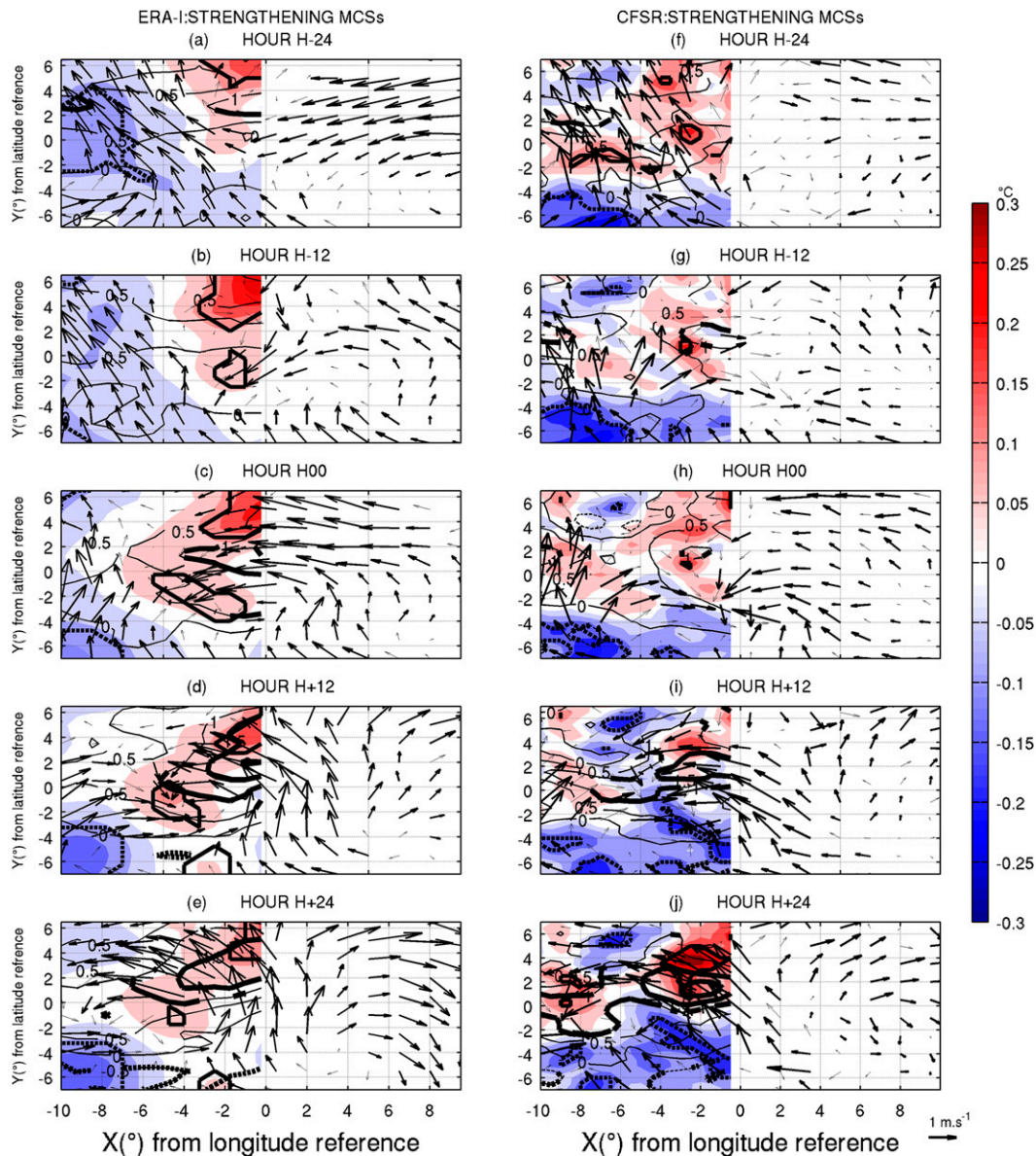
FIG. 14. Strengthening MCSs composite case: composite of SST anomaly (colors, ^{\circ}\text{C} ), anomaly of the vertical integration of specific humidity in the surface–850 hPa layer (contours, \text{kg m}^{-2} ), and surface wind anomaly (arrows, \text{m s}^{-1} ) at (a),(f) H - 24 h, (b),(g) H - 12 h, (c),(h) H00 , (d),(i) H + 12 h, and (e),(j) H + 24 h with (left) ERA-Interim and (right) CFSR. Significant values are in black bold contours for the SST anomaly and in bold arrows for the surface wind anomaly.
