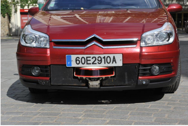
Fig. 4. Vehicle Carmen with Alaska XT lidar embedded in the front bumper.
