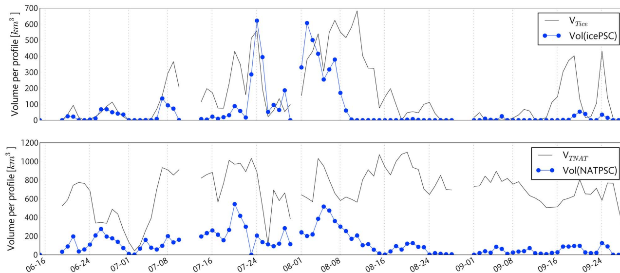
Figure 16. Simultaneous evolution during the 2006 Antarctic winter of volumes with stratospheric temperatures below the frost point (line) and volumes of PSC (dots), for (top) ice and (bottom) NAT particles using the intersection of WRF model output with CALIOP observations.
