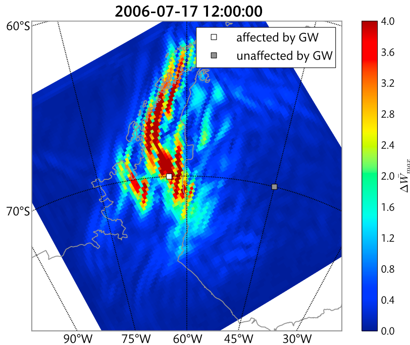
Figure 1. Map of the geographic distribution of the maximum variation of vertical wind speed (m/s) across the vertical dimension of the simulated domain (10–120 hPa) on July 17th, 2006 at 12:00UTC. Coordinates for the domain corners are 85.1°W, 64.9°S (top left), 54.4°W, 59.5°S (top right), 27.3°W, 69.7°S (bottom right) and 76.9°W, 80.4°S (bottom left).
