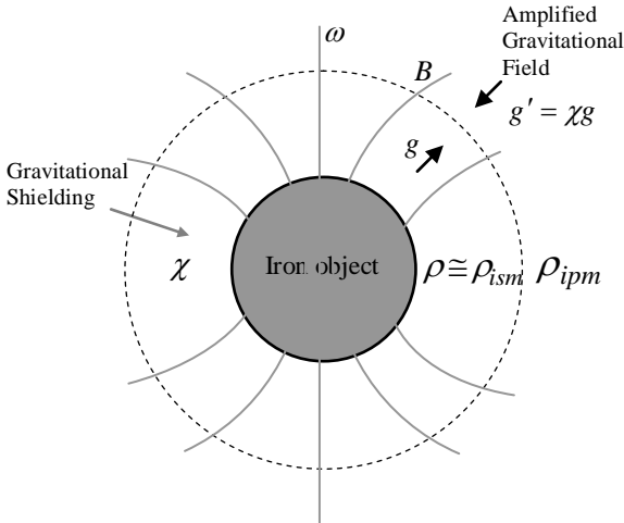
Fig. 1 – Inversion and Amplification of the Gravitational Field . The gravitational field produced by the rotating iron object, g (repulsive), is inverted and amplified by the gravitational shielding (region with density \rho \cong \rho_{ism} , between the iron object and the dotted circle). Thus, out of the gravitational shielding the gravity acceleration becomes attractive, with intensity: g' = \chi g .
