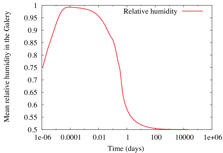
Figure 6: Four fractures test case: mean relative humidity in the gallery as a function of time (equal to 0.5 at initial time).
