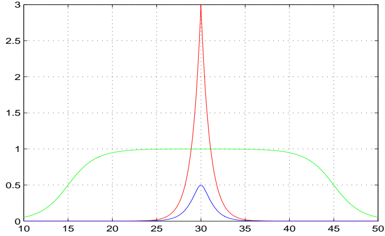
Figure 4: Localization-function \phi_{green}(x) = \psi(x - 15) - \psi(x - 45) (at time t = 10 ) profile. Also, the peakon 3\varphi(x - 30) and the smooth-peakon 3\rho(x - 30) (at time t = 10 with speed c = 3 ) profiles. In this example, one can see that \phi_{green} is close to 1 on ]20, 40[ , and decays exponentially on \mathbb{R} \setminus ]10, 50[ .
