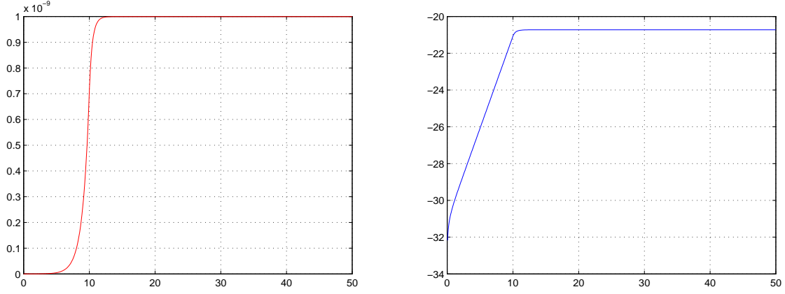
Figure 2: Distance between two very close peaks (at time t = 10 with respective speeds 1 and 1+10^{-10} ).
