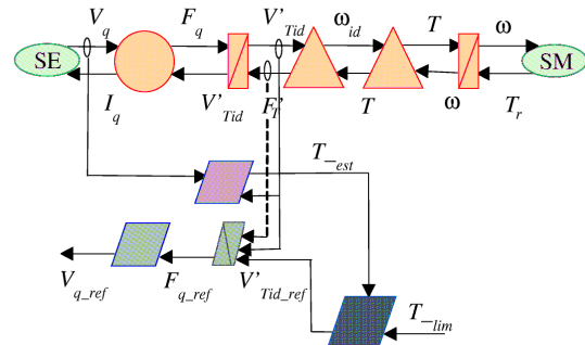
Fig. 9. Control structure for an active claw application.
