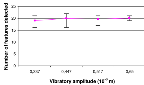
Fig. 17: interpretation of standard deviation error rate for 21 features
