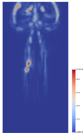
Figure 12: Relative difference between numerical enthalpies with \lambda = 0 and \lambda \neq 0 at time t = 0.55 s (test case of § 5.4.3, EOS : NIST-p)
