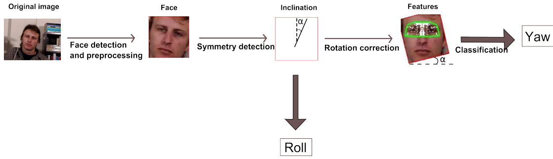
Fig. 1 Proposed approach.
