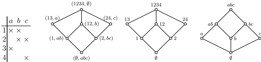
Fig. 1. From left to right: The incidence table of a context, its concept lattice, the lattices of extents, and the lattice of intents
