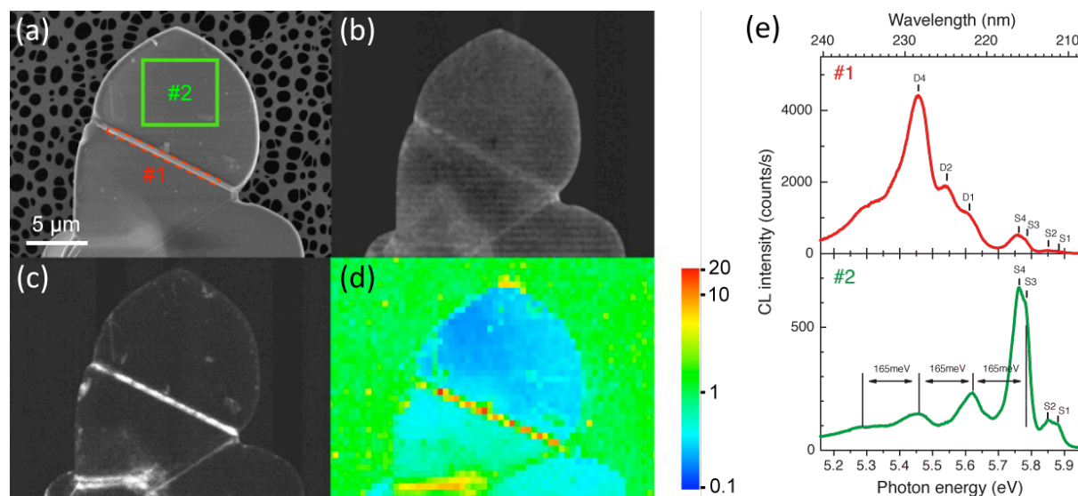
Figure 1: (a) SEM image of a h-BN crystallite; (b), (c) Corresponding CL images recorded (b) on the main S line (S3-S4), and (c) on the main D line (D4). (d) Map of the D/S ratio. (e) CL spectra recorded in the areas #1 (grain boundary) and #2 (middle of the grain), indicated in (a).
