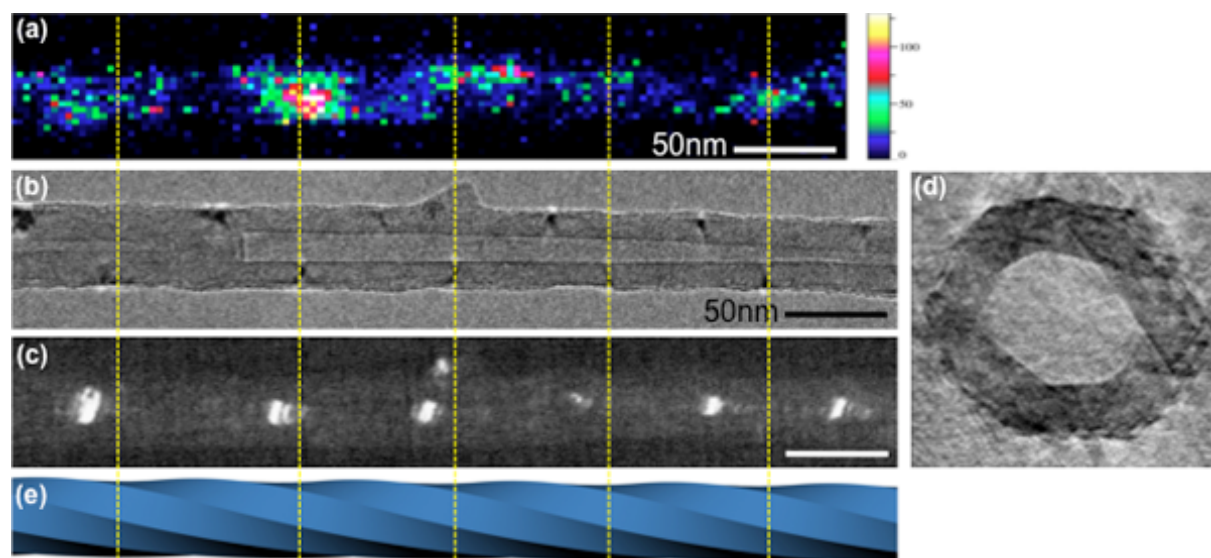
Figure 2: Images of a BN nanotube: (a) 3nm spatially resolved CL image recorded at 5.49 eV (226 nm); (b), (c) Corresponding TEM images in (b) bright-field mode, and (c) dark-field mode on the (100) reflection. (d) Heptagonal tube cross-section obtained by tomography experiment. (e) Structure of the tube as deduced from (b-d) images.
