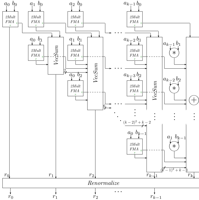
Fig. 4: Multiplication of FP expansions with k terms. Each 2MultFMA box performs Algorithm 2, the product is outputted downwards and the error to the right; the VecSum box performs Algorithm 3, in which the most significant component of the sum is outputted downwards; the circled + and * signs represent standard round-to-nearest FP addition and multiplication.
