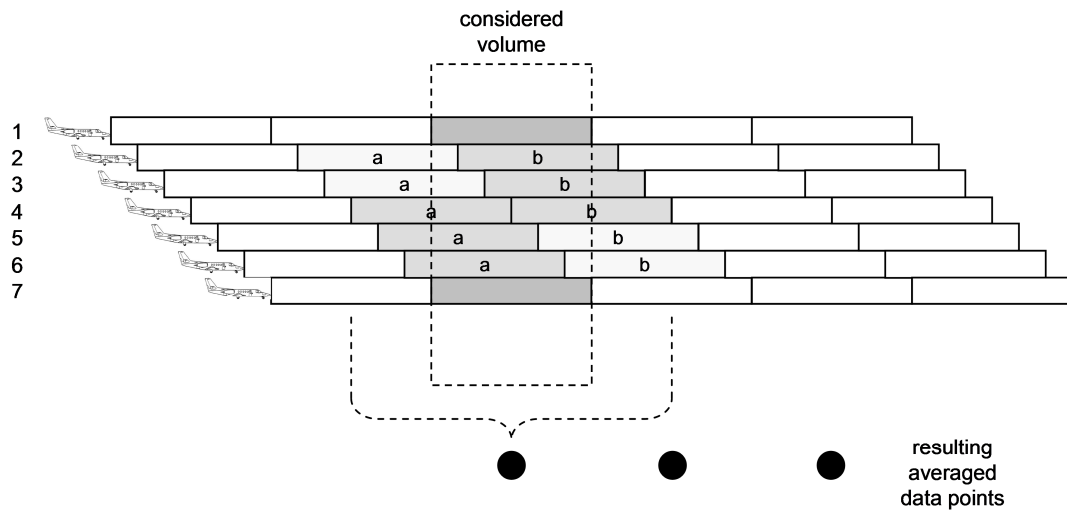
Figure 18 Averaging of various shots in a volume of length Dr
