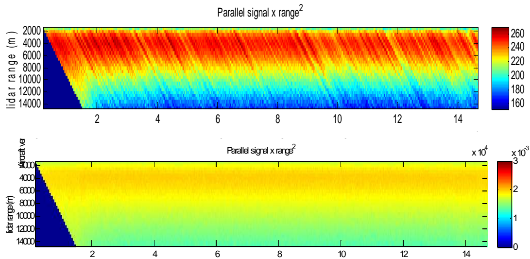
Figure 21: Normalization effect on averaged parallel signal multiplied by the squared range (zone 20 - flight9). top: without normalization, bottom : with normalization
