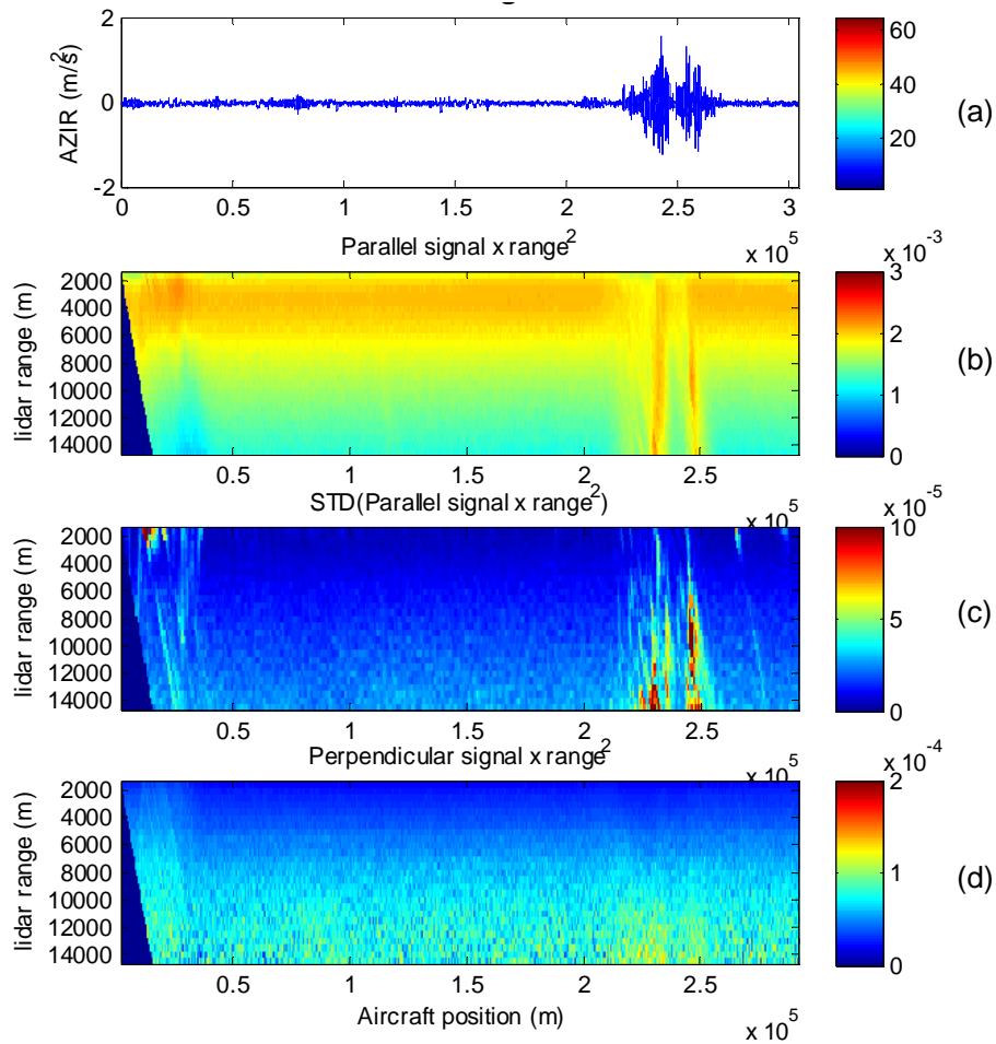
Figure 22: Pre-processed lidar data for area 5: (a) vertical acceleration, (b), parallel signal \times range^2 , (c) standard deviation calculated on parallel signal, (d) perpendicular signal \times range^2 .
