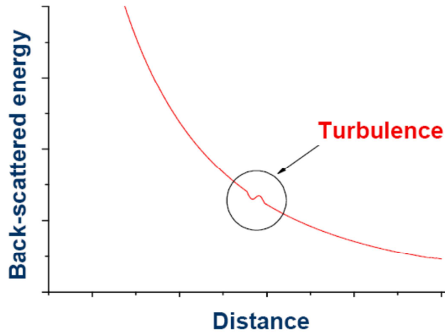
Figure 3: Principle of a LIDAR based turbulence detection (without noise, the shown turbulence effect being greatly exaggerated and simplified)
