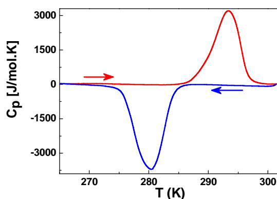
Figure 3. DSC curves for [\text{Fe}(\text{hyetrz})_3]\text{I}_2 \cdot \text{H}_2\text{O} over the temperature range 265-303 K.
