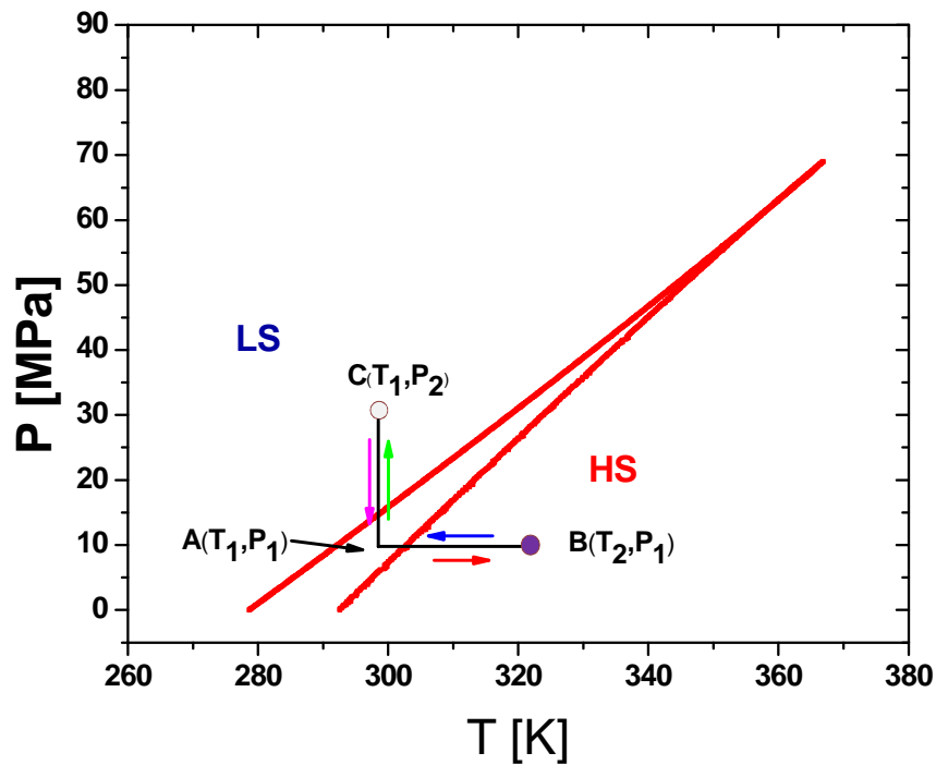
Figure 7 Pressure-temperature phase diagram calculated for a SCO system switching around the room temperature region using the following parameters values: \Delta_0/k_B=1978.6K , \delta V=100\text{\AA}^3 , \ln g = 6.906 and T = 360 K.
