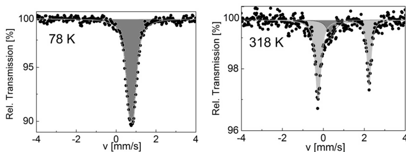
Figure 4. ^{57}\text{Fe} Mössbauer spectra for [\text{Fe}(\text{hyetrz})_3]_2 \cdot \text{H}_2\text{O} at 78 K (left) and 313 K (right).
