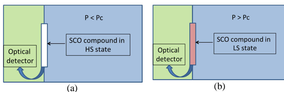
Figure 1 SCO material used as pressure sensor: (a) the SCO material reflects the light to the detector, indicating that the pressure is below the critical point; (b) the SCO material does not reflect the light to the detector, indicating that the pressure is above the critical point.
