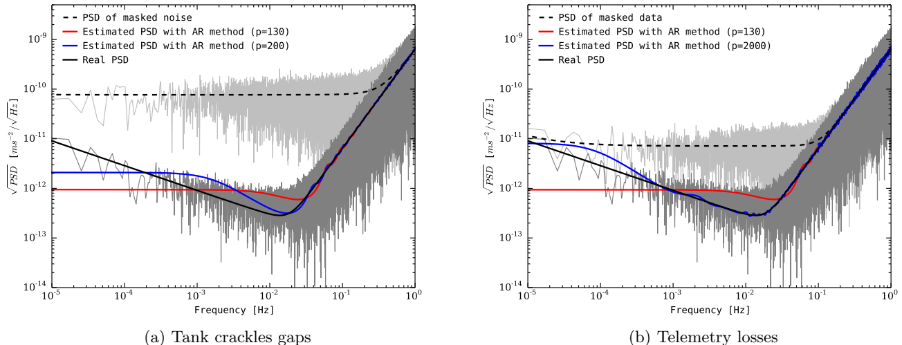
FIG. 4. PSD estimates of the noise in presence of missing data. The black dashed curve is an estimate of the masked data PSD [obtained using Eq. (??)], the black solid curve is the actual noise PSD, and the red and blue curves are the PSD estimates of the AR model obtained with Burg’s algorithm. The periodograms of the regression residuals are also plotted for the complete (dark grey) and masked (light grey) cases.
