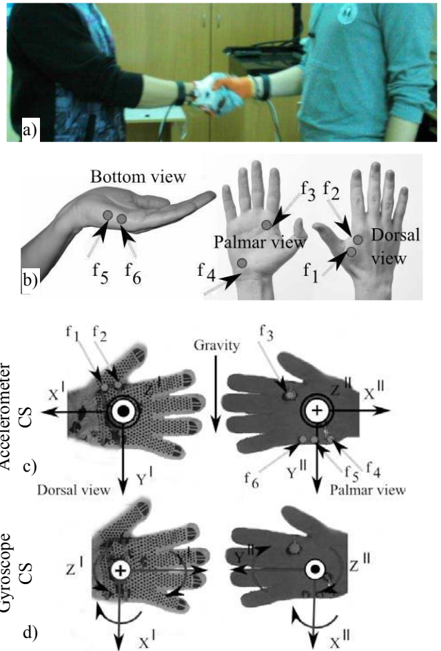
Figure 1. Two interacting subjects carrying the prototype system. a) the data gloves (subjects I and II); b) the six force sensitive resistors (above sensors position on the hand is shown); c) local coordinate system (CS) for accelerometers; d) local coordinate system for gyroscopes.
