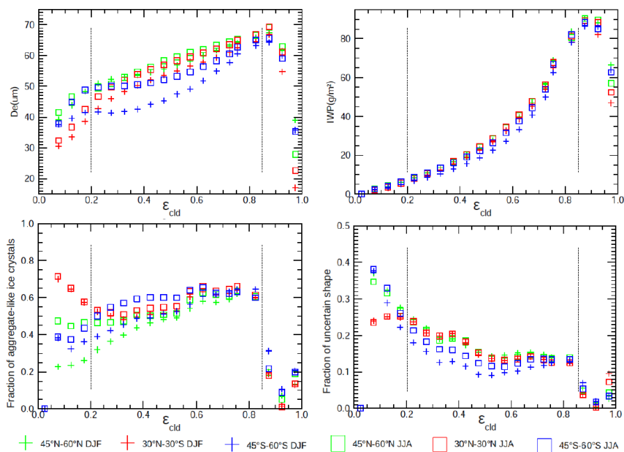
Fig. 4. Bulk microphysical properties as function of cloud emissivity, averaged over the period 2003–2009. Crosses and squares represent averages over boreal winter and over boreal summer, respectively. Green symbols are for NH midlatitudes, red for the tropics and blue for SH midlatitudes. The vertical lines represent the emissivity boundaries between which the microphysical property retrieval is applied.
