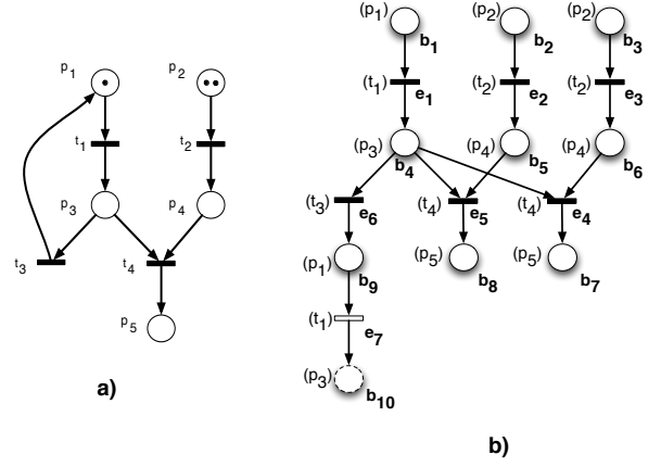
Figure 3: a) Petri net, b) Unfolding
