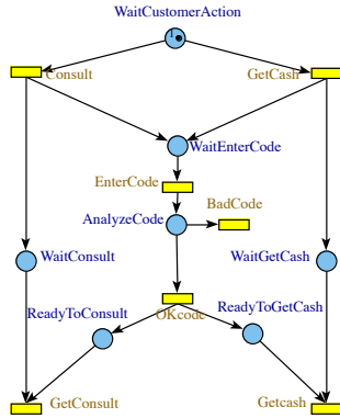
Figure 8: Cashdispenser
