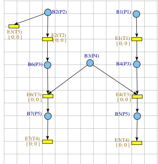
Fig. 5. Unfolding
