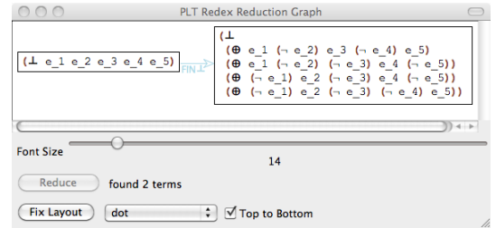
Fig. 6. (\perp e_1 e_2 e_3 e_4 e_5)
