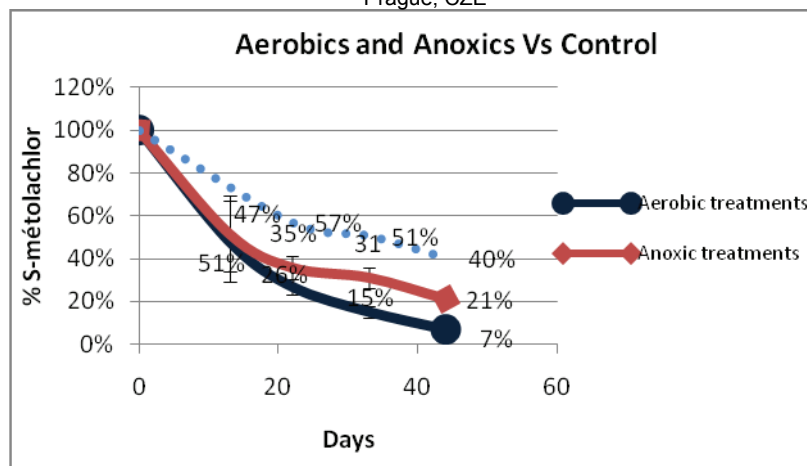
Figure 3. Remaining S-metolachlor in aqueous phase means for treatments in Aerobic ● and Anoxic ◆ conditions Vs the abiotic control.
